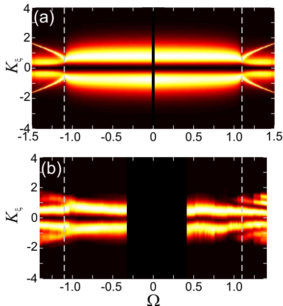
FIG. 4: (color online) (a) Same as for Fig.3 but computed for |\tilde{p}_r|^2 + |\tilde{p}_r^*|^2 . The vertical dashed line separates the snake ( |\Omega| < 1.08 ) from the oscillatory snake ( |\Omega| > 1.08 ) regimes. (b) Experimental results.
