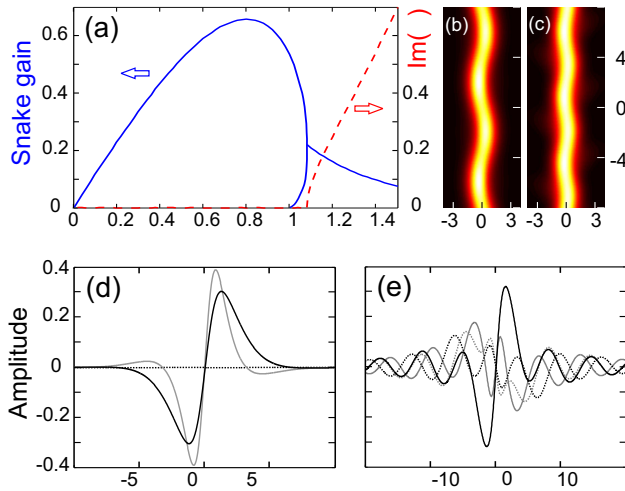
FIG. 1: (color online) (a) Snake instability gain g = 2\text{Re}(\Gamma) (solid blue line) and imaginary part of \Gamma (dashed red line) plotted as a function of the perturbation frequency \Omega . Beyond the frequency cut-off \Omega_c \approx 1.08 , \Gamma is complex and the snake instability becomes oscillatory. (b)-(c) Density plot of the spatiotemporal intensity profile for \epsilon_0 = 1 and \Omega = 0.8 and 1.2 , respectively. (d)-(e) Eigenfunctions U (gray) and V (black) plotted as a function of the transverse coordinate \xi below (b) and above (c) \Omega_c . Solid lines stand for the real part and dashed lines for the imaginary part. Figures adapted from [5].
