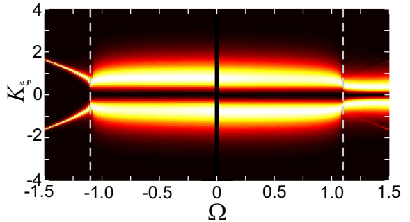
FIG. 3: (color online) Density plot of the theoretical evolution of the angularly resolved spectrum |\tilde{p}_r|^2 as a function of the frequency \Omega . Each spatial spectra (i.e. each profiles for a given frequency \Omega ) has been normalized to unity. Brighter colors stand for larger amplitudes. The vertical dashed lines separate the snake ( |\Omega| < 1.08 ) from the oscillatory snake ( |\Omega| > 1.08 ) regimes.
