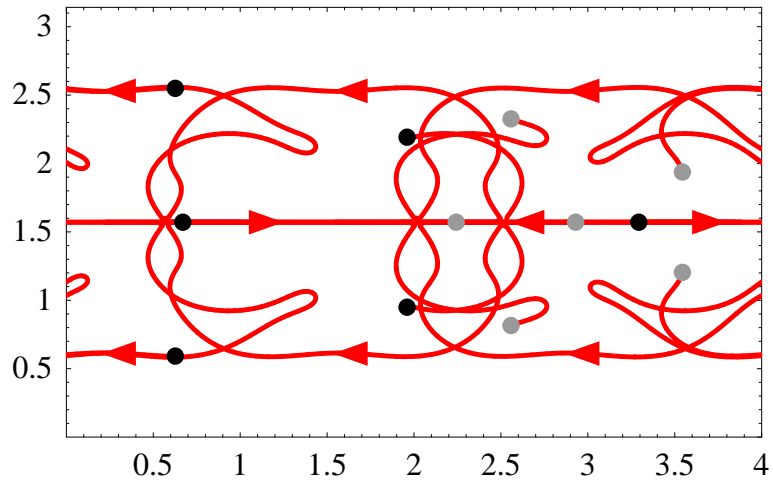
Figure 5.5: The pole dynamics of a (3 : 2 : 1) -solution. The black dots mark the initial position of the poles; the grey dots mark the position of the poles at t = 0.4 .
