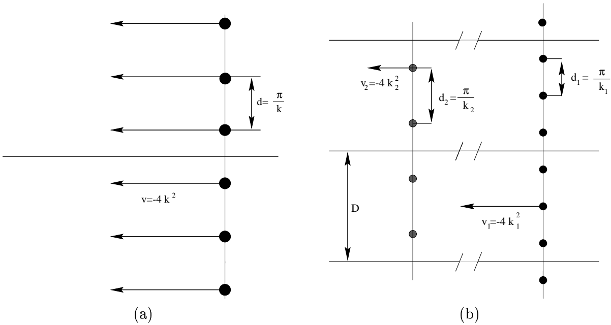
Figure 2.1: (a) The motion of the poles of a one-soliton solution in the complex plane. (b) The asymptotic motion of the poles of a two-soliton solution.
