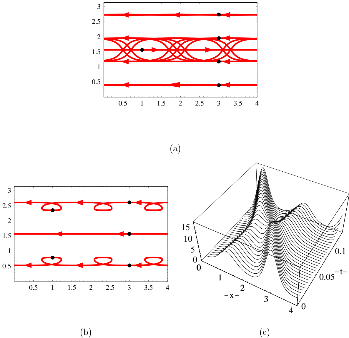
Figure 5.4: N = 5 : (a) The pole dynamics of a (4 : 1)-solution in the fundamental domain. (b) The pole dynamics of a (3 : 2)-solution in the fundamental domain. (c) The KdV solution u(x, t) corresponding to the pole dynamics in (b). In (a) and (b), the initial positions of the poles are indicated. Both solutions are quasiperiodic in time. u(x, t)
