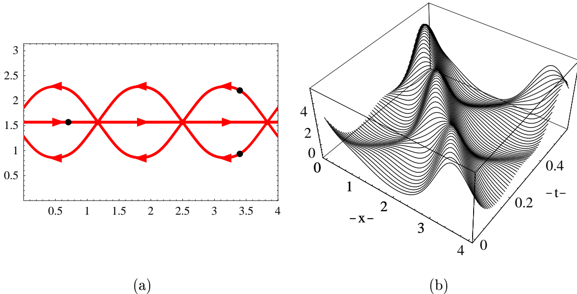
Figure 5.1: The solution of Dubrovin and Novikov, with L_1 = 4 and L_2 = \pi . (a) The motion of the poles in the fundamental domain. The initial position of the poles is indicated by the black dots. The arrows denote the motion of the poles. (b) The KdV solution u(x, t)
