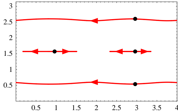
Figure 5.2: N = 4 : the pole dynamics of a (3 : 1) -solution. The initial positions of the 4 poles are indicated. The arrows on the centerline indicate that the poles there move in both directions.
