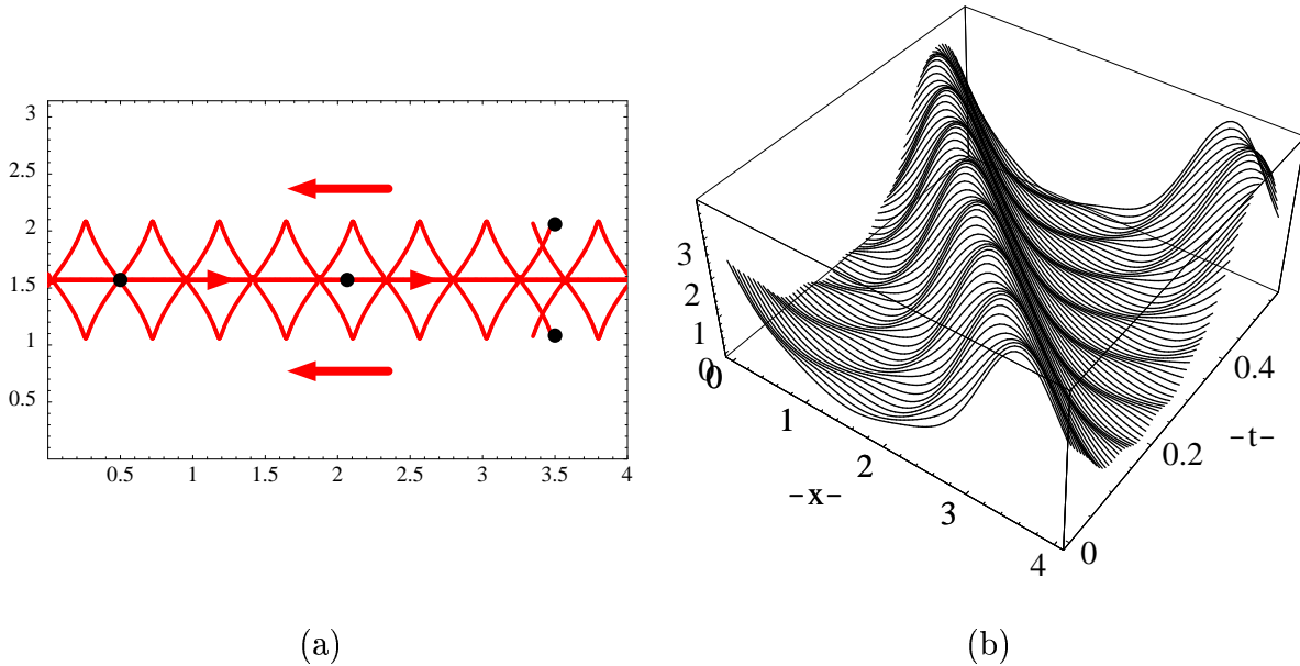
Figure 5.3: An N = 4 , M = 2 Treibich-Verdier solution, with L_1 = 4 and L_2 = \pi . (a) The motion of the poles in the fundamental domain. The initial position of the poles is indicated by the black dots. The initial time t = 0 was chosen different from the collision times t_c . The arrows denote the motion of the poles. (b) The KdV solution u(x, t)
