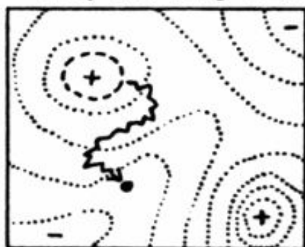
D. Close Inbreeding 4NU, 4NS very small
