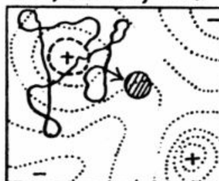
E. Slight Inbreeding 4NU, 4NS medium
