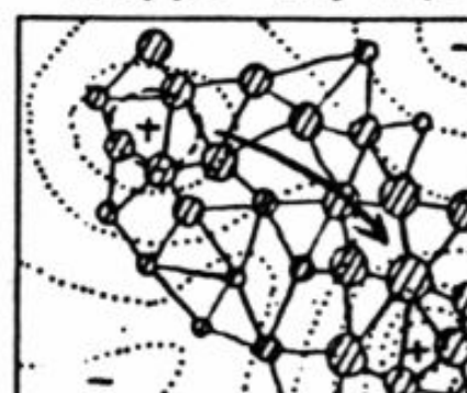
F. Division into local Races 4nm medium
