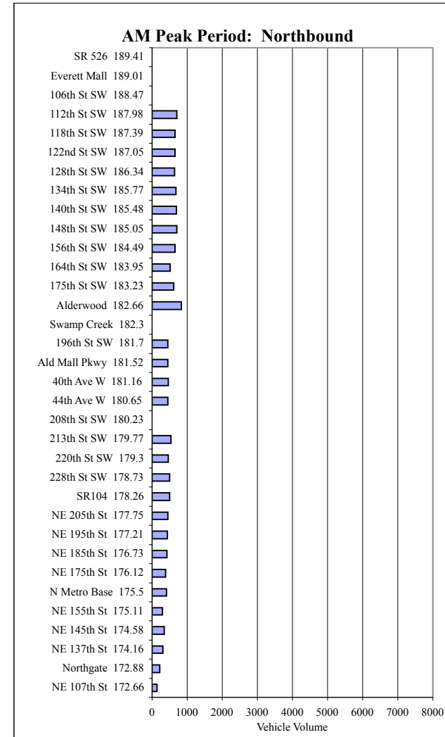
HOV Traffic Flow Profile (2003): I-5 North of the Seattle CBD During the AM Peak Period
