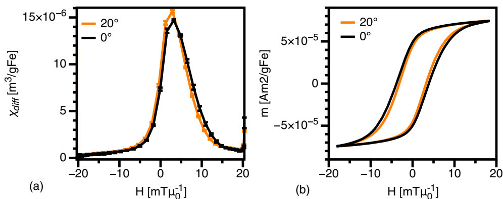
FIG. 8. (Color online) MPS (26 kHz, 20 mT/ \mu_0 ) response of SPIOs in water at room temperature and 0°C (liquid state). Error bars in (a) represent the standard deviation of three measurements.
