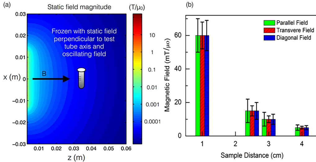
FIG. 3. (Color online) (a) The simulated magnetic field of the permanent magnet (lines of equal field strength are shown in the figure). The test tube containing the SPIOs was frozen in this orientation at various distances to achieve the varying magnetic field amplitudes. In the example illustrated in (a), the aligning field was applied perpendicular to the direction of the oscillating (drive) field, which was always applied parallel to the long axis of the sample tube. The surface field for these magnets is 0.12 T, so we see that at 5 cm the field is in the single millitesla range as shown in experiment. Notably at this distance we can see the variations in the field are minimal within the test tube. (b) Measured variation of field strength with distance from the magnet. Error bars represent the variation in field within the sample tube for the stated field orientation, and they differ because the tube geometry is anisotropic.
