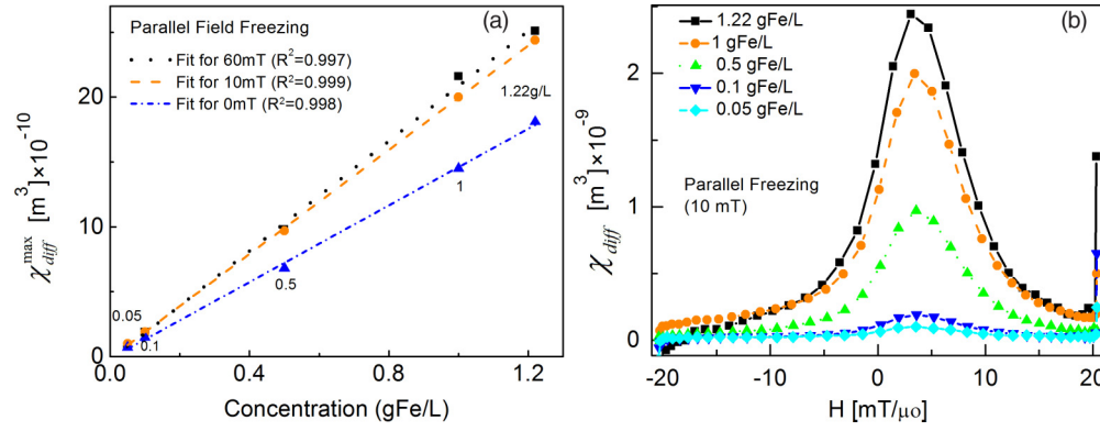
FIG. 9. (Color online) \chi_{diff}^{max} data (at 26 kHz and 20 mT/\mu_0 ) of different concentrations: (a) at different freezing fields and (b) at 10 mT/\mu_0 parallel freezing.
