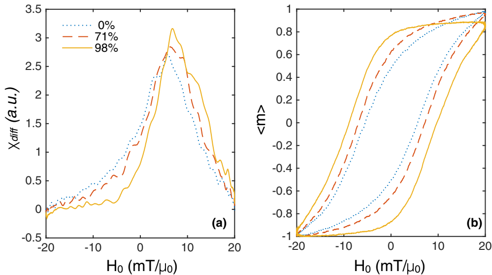
FIG. 12. (Color online) Magnetizations were simulated using a 40-kHz, 20 \text{mT}/\mu_0 field at room temperature to show how the (a) differential magnetic susceptibility in arbitrary units \chi_{\text{diff}} (arb. units) and (b) hysteresis loops are affected by increasing the percentage of particles aligned in the direction of the applied field. The size and anisotropy distribution are identical to that in other simulations.
