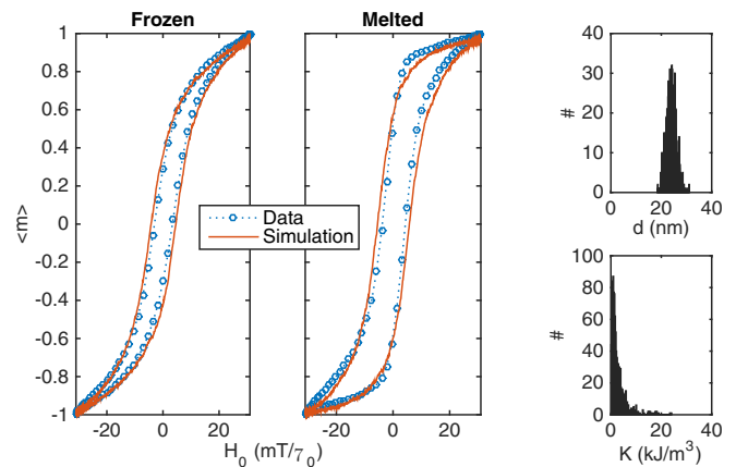
FIG. 11. (Color online) Comparison between simulation and experiment for nanoparticles either in either a frozen or melted state. Spectroscopy was performed with a 26-kHz, 31 mT/\mu_0 field. The log-normal distributions of particle diameter and anisotropy constant are shown on the right by number in a representative 1000-particle subsample.
