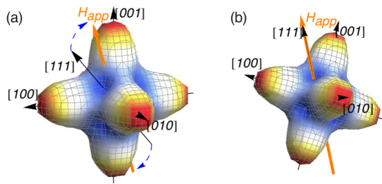
FIG. 1. (Color online) The magnetocrystalline energy surface for cubic magnetite (negative K_1 ), which has easy directions in the [111] family. After (a) applying an arbitrary magnetic field vector H_{\text{app}} in a fixed direction, particles in solution undergo Brownian rotation through a small angle until (b) the nearest easy axis is aligned with the applied field.
