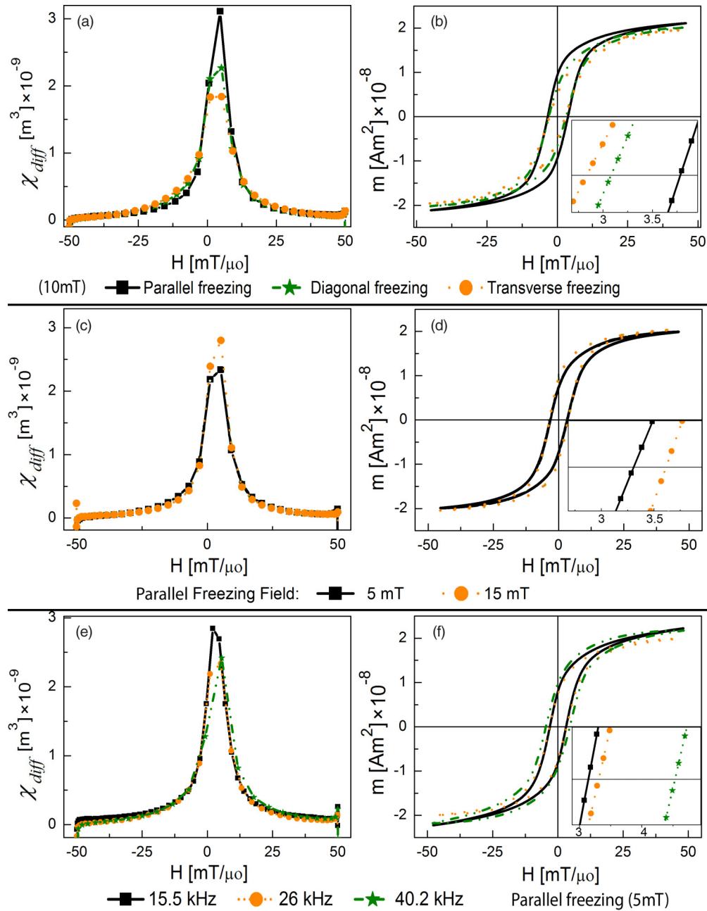
FIG. 6. (Color online) MPS (26 kHz, 50 mT/ \mu_0 ) signal parameters of MNPs, field frozen (10 mT/ \mu_0 ) along different directions with respect to the MPS applied field. (a) \chi_{diff} and (b) integrated m(H) curves. MPS (26 kHz, 50 mT/ \mu_0 ) signal parameters of MNPs, frozen in different magnetic fields along parallel orientation: (c) \chi_{diff} and (d) m(H) curves. MPS (50 mT/ \mu_0 , different frequencies) signal parameters of MNPs, frozen in 5 mT/ \mu_0 along parallel orientation: (e) \chi_{diff} and (f) m(H) curves.
