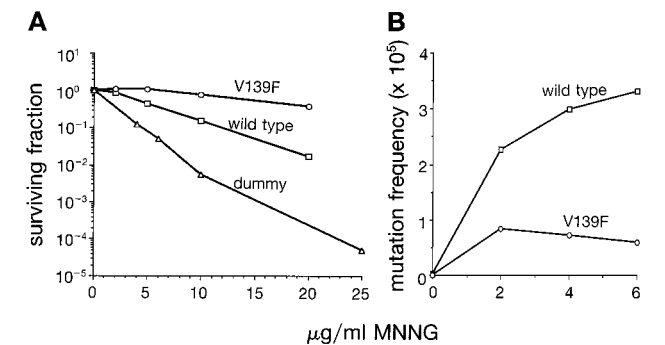
FIG. 4. MNNG-induced cytotoxicity and mutagenesis. GWR111 cultures containing the dummy vector (see Materials and Methods) or plasmids expressing either the wild-type or mutant V139F human MGMT were treated with graded amounts of MNNG and spread on (A) growth media plates to determine survival or (B) plates containing 100 μg/ml rifampicin to determine mutation frequency (not done for dummy strain). Average values of at least two independent experiments are shown. □, wild type; ○, V139F; (Δ) dummy.
