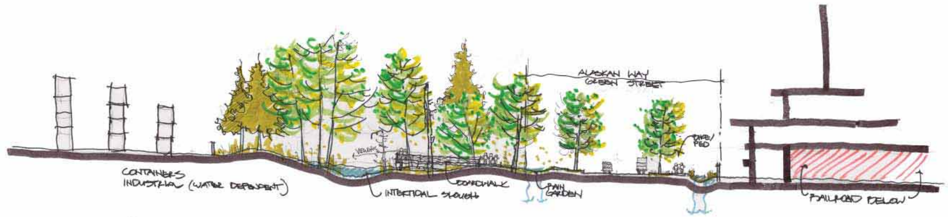
SECTION @ ALASKAN WAY CONTAINER CANYON 1" = 20'
