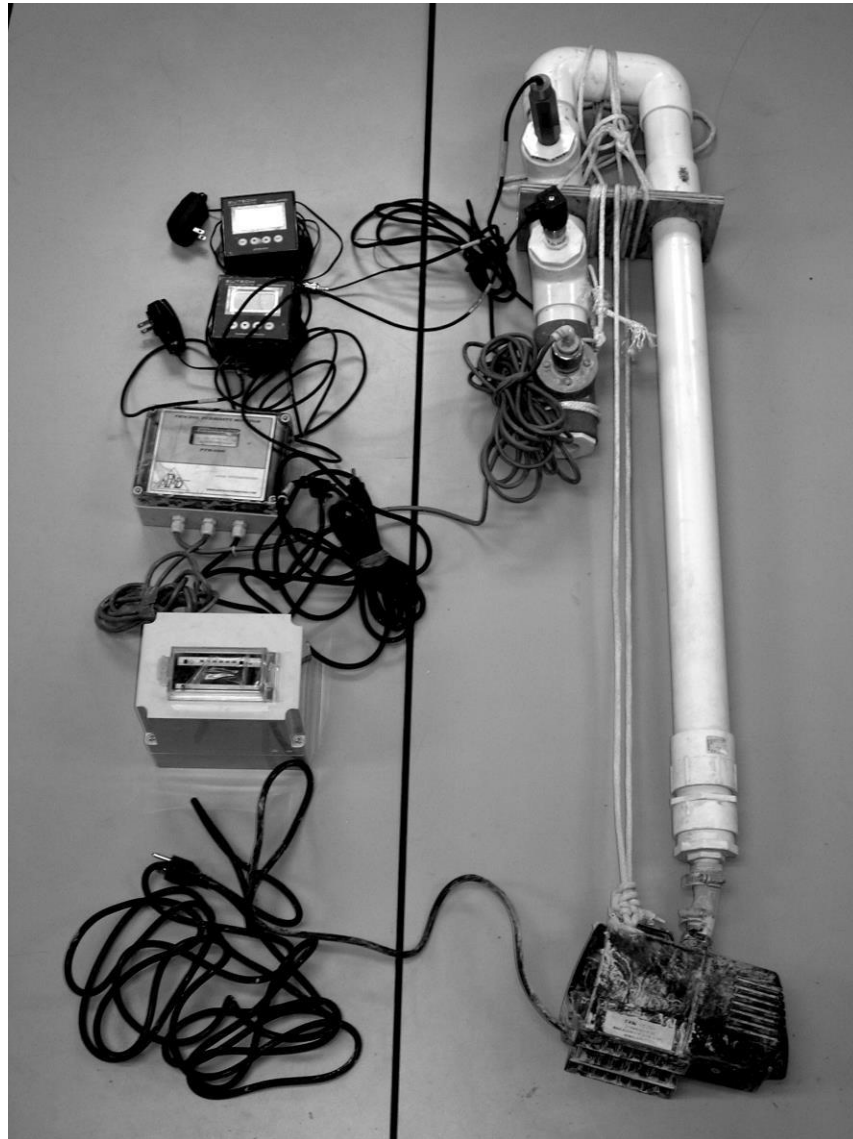
Figure 4.1 Sensor Assembly.
