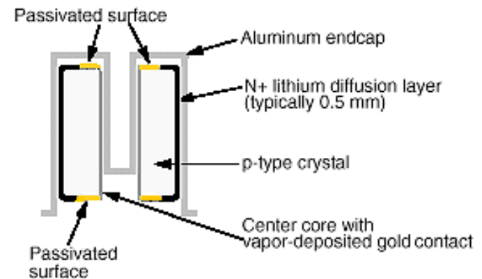
Ge detector with well for small samples
