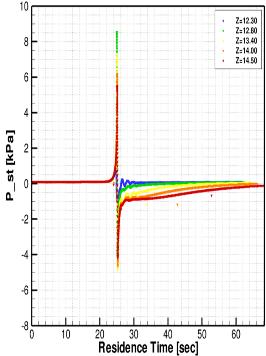
Static pressure history on particles injected at inlet (X,Y)=(0,50) in the inlet along tidal channel
