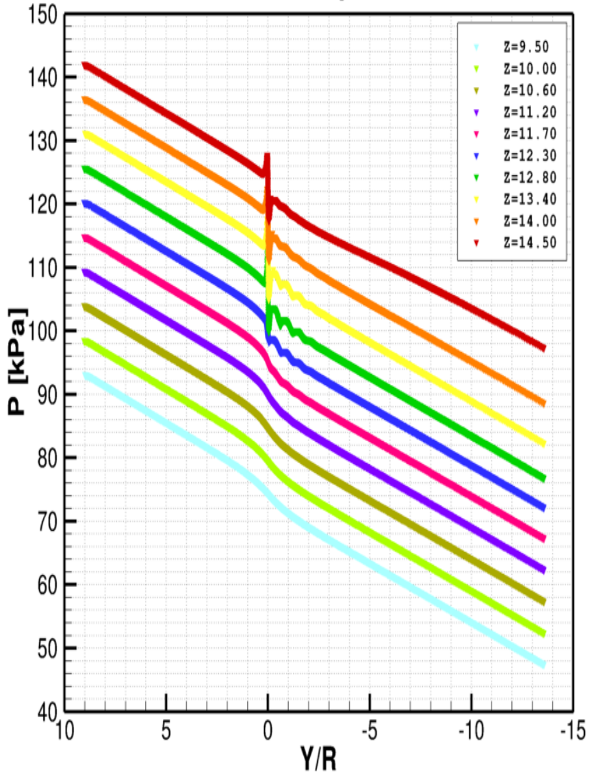
Static pressure (including hydrostatic pressure) history on particles injected at (X,Y)=(0,50) in the inlet along the channel.
