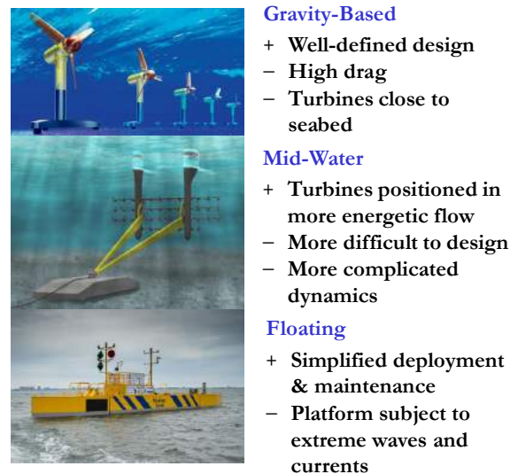
FIGURE 1. FOUNDATION DESIGN ALTERNATIVES [8-10].
