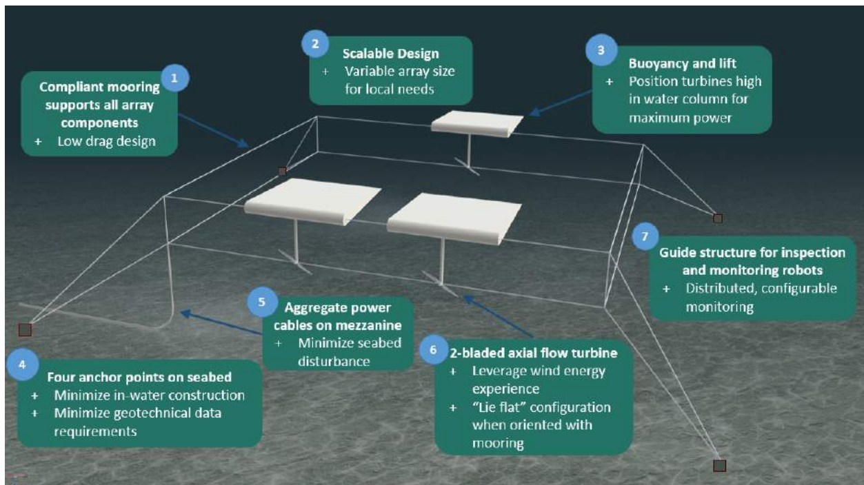
FIGURE 3 MEZZANINE MOORING CONCEPT [18]
