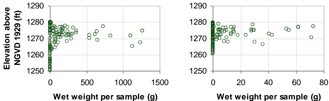
Figure 5. Wet weight of macrophytes by depth for samples collected from Spokane arm (left) and mainstem (right) reservoir sites. Note the different biomass scales.
