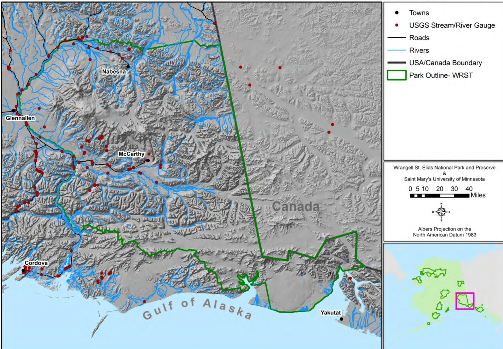
Plate 44. USGS stream and river gauge sites, WRST.
