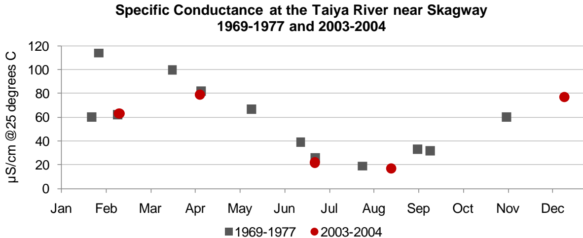
Figure 33. Specific conductance at the Taiya River near Skagway: 1969 to 1977 and 2003 to 2004 (USGS 2010b).
