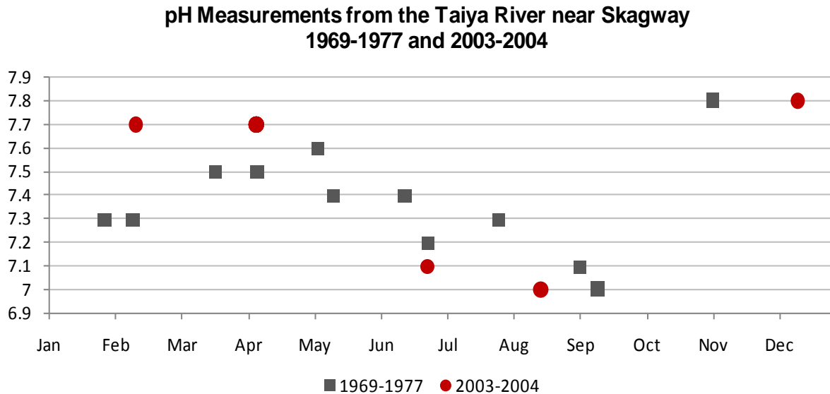
Figure 32. pH measurements from the Taiya River near Skagway: 1969 to 1977 and 2003 to 2004 (USGS 2010b).
