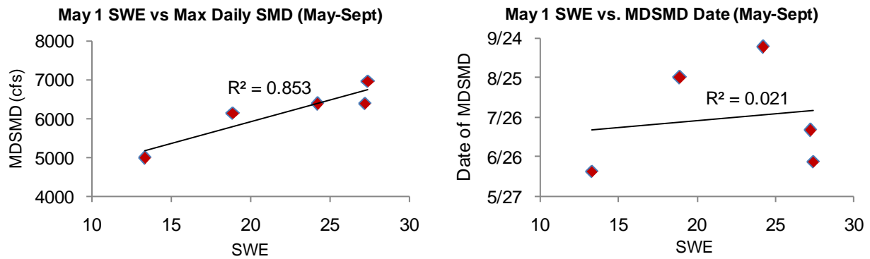
Figure 52. Taiya River near Skagway: 1 May snow water equivalent (SWE) at the Moore Creek Bridge SNOTEL station versus maximum daily snowmelt discharge (left) and the date of maximum daily snowmelt discharge (right) (USGS site 15056210) (NRCS 2009, USGS 2010a). Maximum daily snowmelt discharge was calculated using May through September. Note: The Moore Creek Bridge SNOTEL station is not in the Taiya river watershed, so results presented above are purely speculative.
