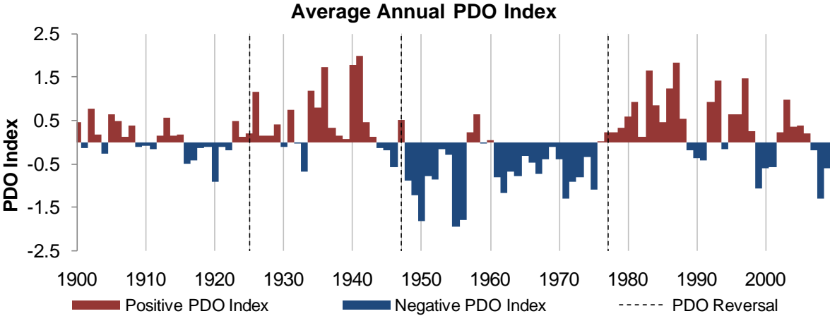
Figure 54. Average annual PDO index, 1900 to 2009 (Mantua 2010b). Vertical dashed lines represent reversals in PDO polarity in 1925, 1947, and 1977.
