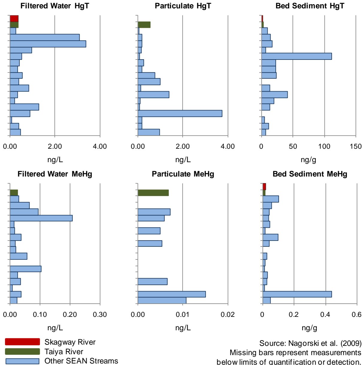
Figure 35. Total mercury (Hg T ) and methylmercury (MeHg) concentrations in filtered water, filter-retained particulates (in the water column), and in bed sediments of the Skagway River (red), Taiya River (green), and other SEAN streams (blue) (Nagorski et al. 2009).
