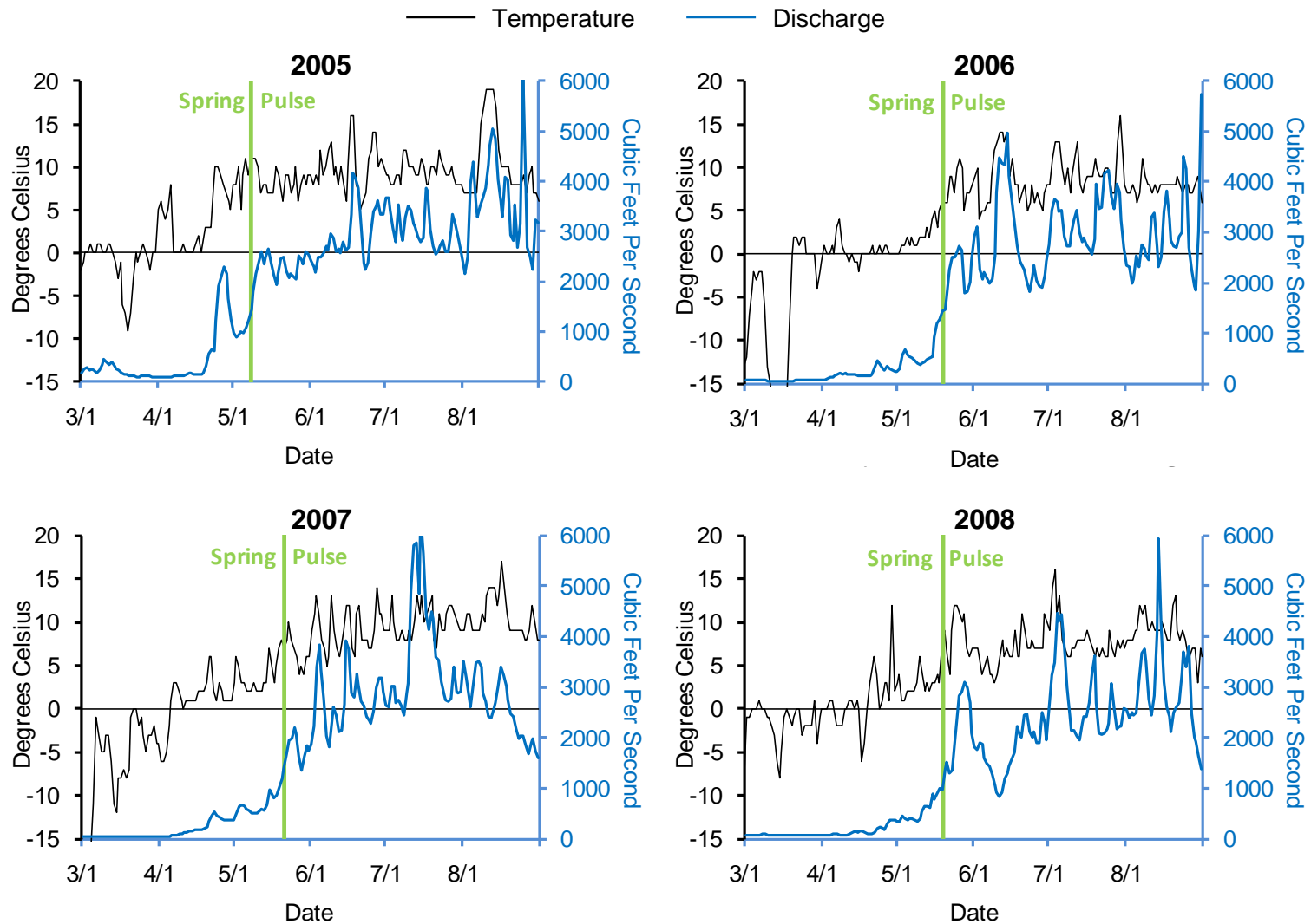
Moore Creek Bridge Daily Mean Temperature and Taiya River Daily Mean Discharge, 2005-2008
