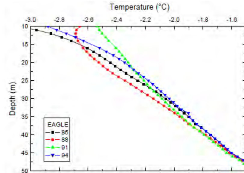
Figure 18. Temperature profiles at the Eagle borehole over time (Osterkamp 2005).
