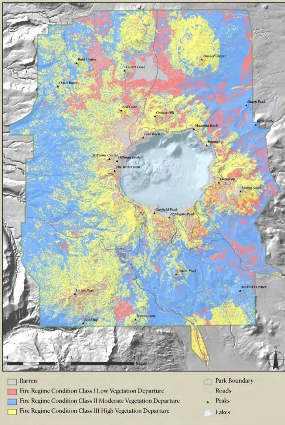
Figure C11. Mapped fire regime condition classes of Crater Lake National Park (LANDFIRE 2008). This map was prepared by other investigators who extrapolated fuels information using Landsat Thematic Mapper and other data. Lands were assigned to map classes by experts in LANDFIRE workshops. The map does not portray fuel, fuel arrangement, or vegetation flammability. The map was based on rough estimates of the level to which fire frequencies have departed from “natural” fire frequencies. FRCC is also not a measure of fire risk or hazard. Increasing FRCC may lead to either more or less severe fire. Nonetheless, FRCC may be useful to identify where fire should be allowed to burn. The natural fire regime of every ecosystem falls into only five classes for determining departure, but the fire regimes of this park do not fit this classification.
