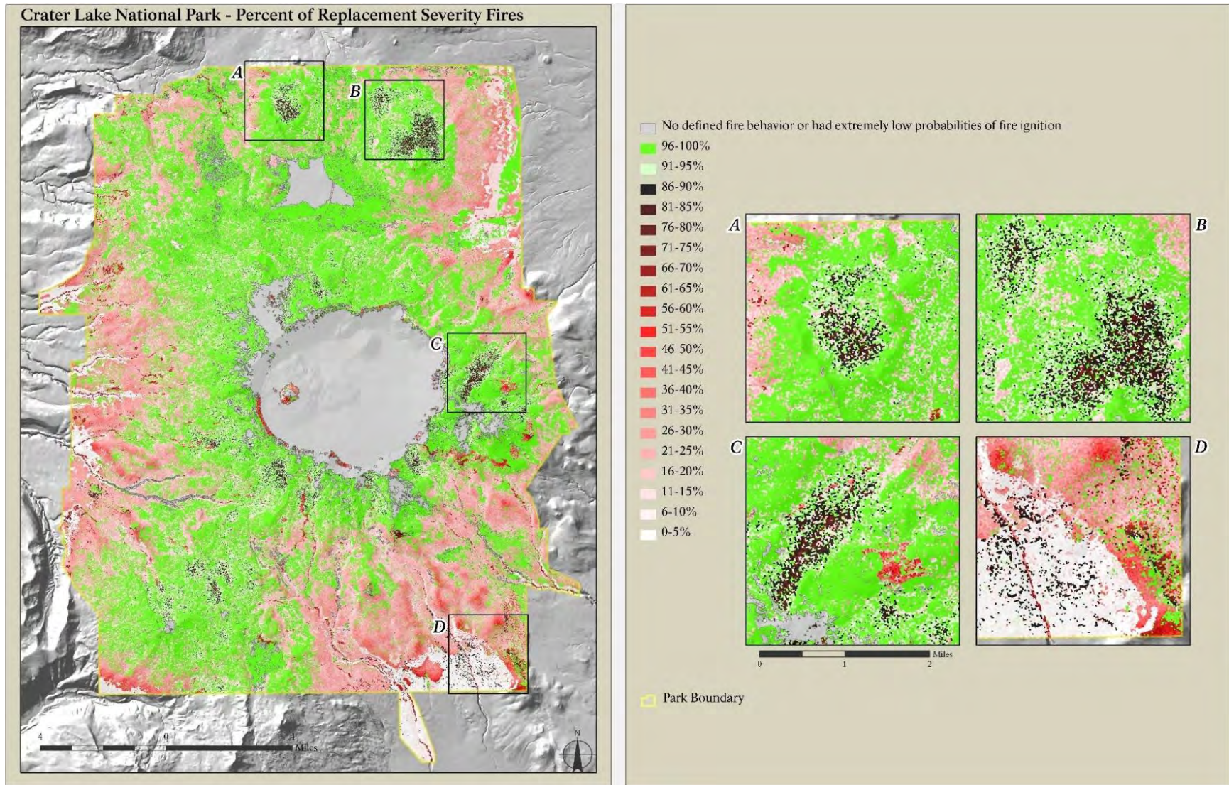
Figure C17. Mapped percent of replacement severity fires of Crater Lake National Park (LANDFIRE 2008). This map was prepared by other investigators who extrapolated fuels information using Landsat Thematic Mapper and other data. Lands were assigned to map classes by experts in LANDFIRE workshops. The map does not portray fuel, fuel arrangement, or vegetation flammability.
