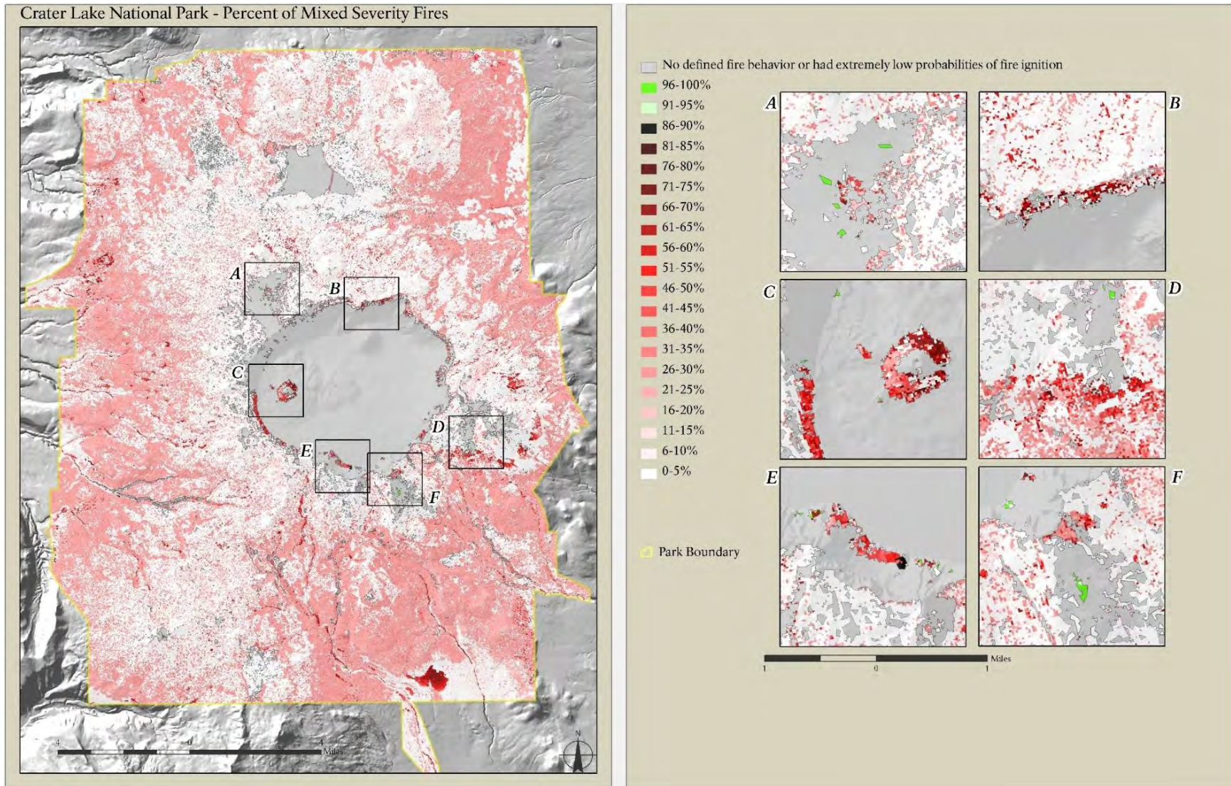
Figure C16. Mapped percent of mixed severity fires of Crater Lake National Park (LANDFIRE 2008). This map was prepared by other investigators who extrapolated fuels information using Landsat Thematic Mapper and other data. Lands were assigned to map classes by experts in LANDFIRE workshops. The map does not portray fuel, fuel arrangement, or vegetation flammability.
