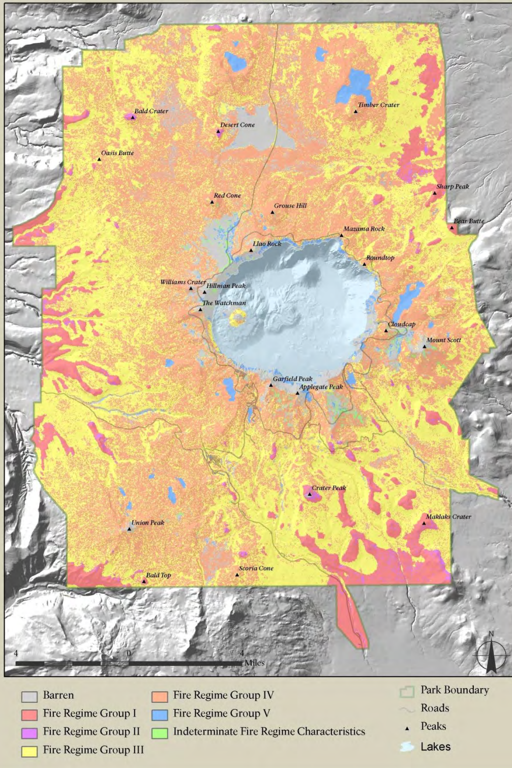
Figure C12. Mapped fire regime groups of Crater Lake National Park (LANDFIRE 2008). This map was prepared by other investigators who extrapolated fuels information using Landsat Thematic Mapper and other data. Lands were assigned to map classes by experts in LANDFIRE workshops. The map does not portray fuel, fuel arrangement, or vegetation flammability.
