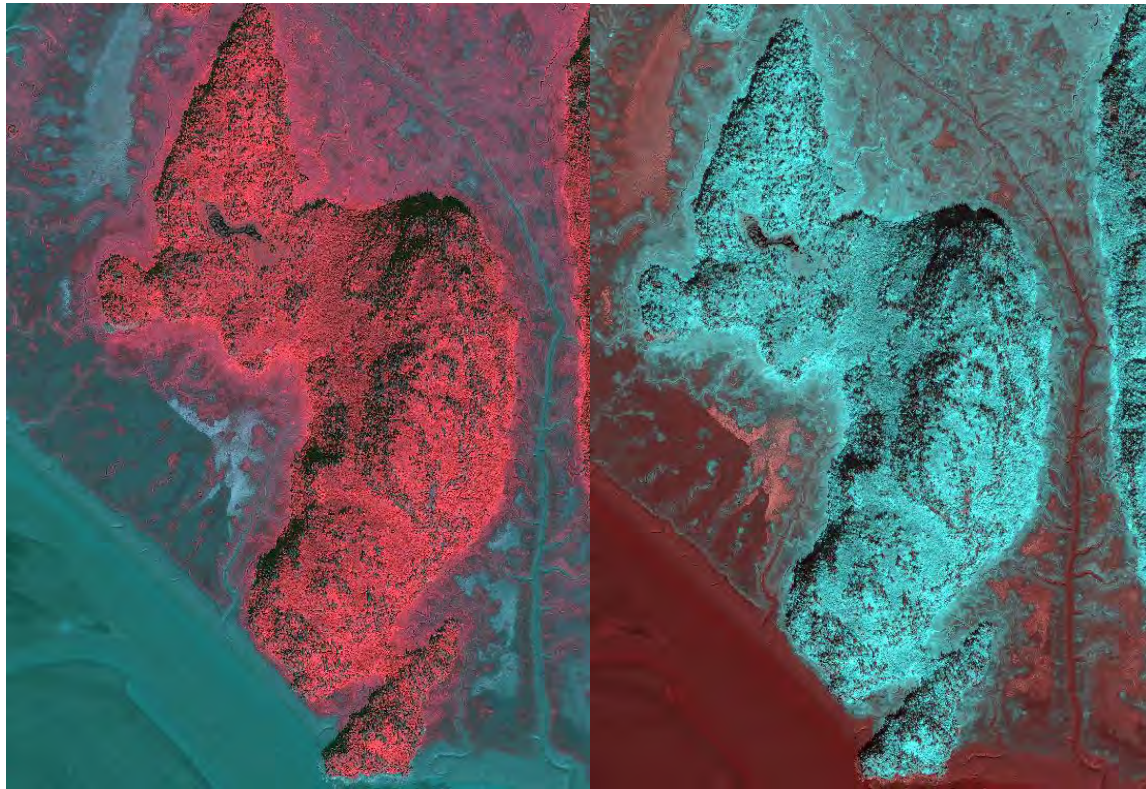
Figure 37. Example of band reordering which provided clarity, LACL.
