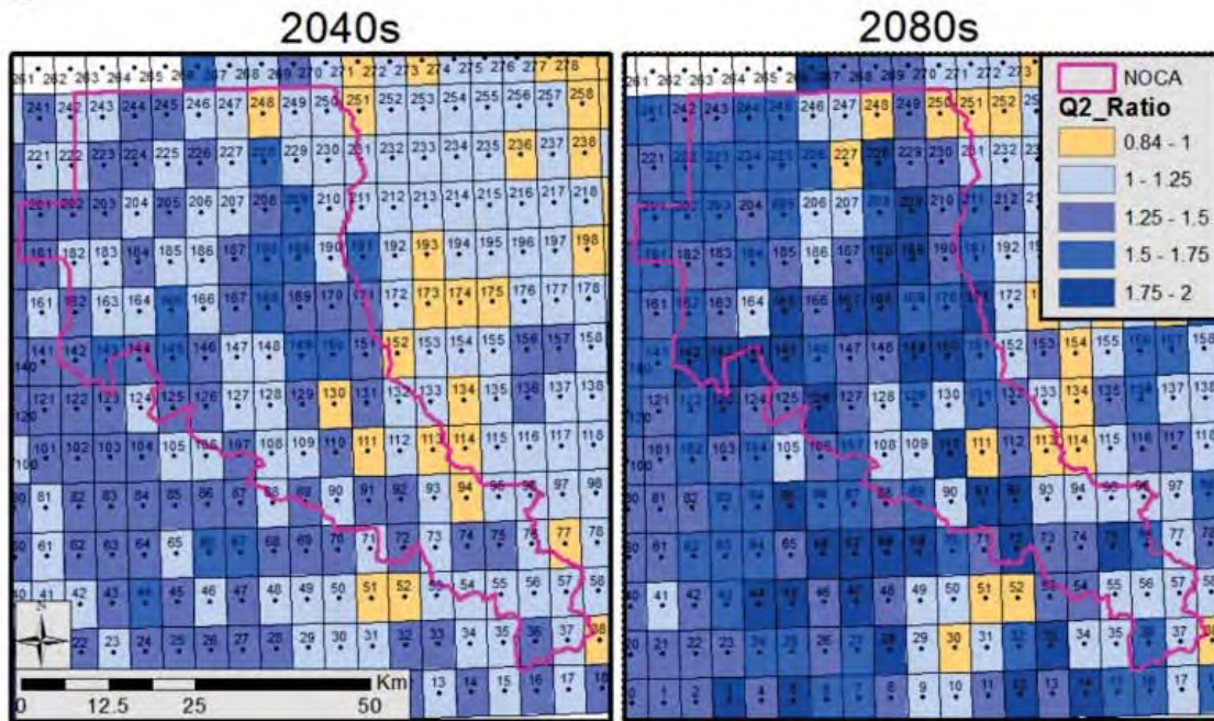
Figure 16. Shifting trend in the ratio of (a) Q100 and (b) Q2 in 2040s (left side) and 2080s (right side) to historical (1916–2006) corresponding peak stream levels. Ratios >1 indicate increasing peak flows in the future (blue). Ratios <1 indicate decreasing peak flows (beige).
