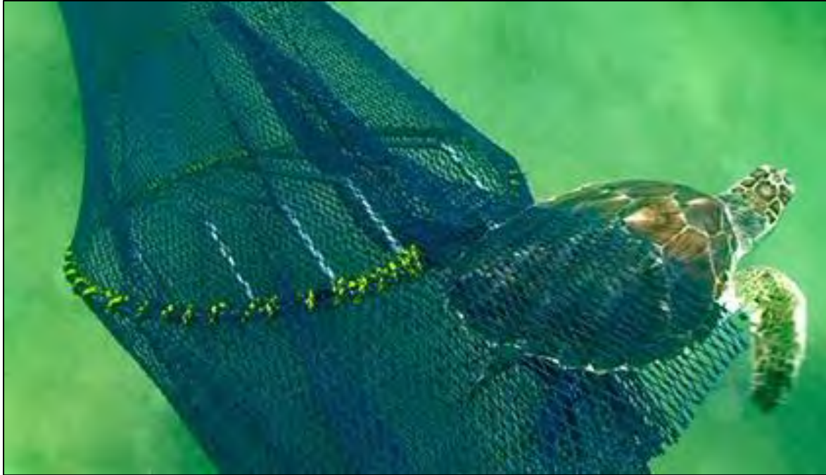
Figure 65. A sea turtle escaping a fishing net through a TED (NMFS photo). Shrimp and other targeted species are small enough to pass through the metal bars, but turtles are stopped and can swim out through a loose mesh opening.
