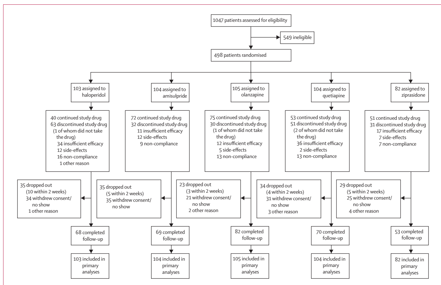
Figure 1: Trial profile
