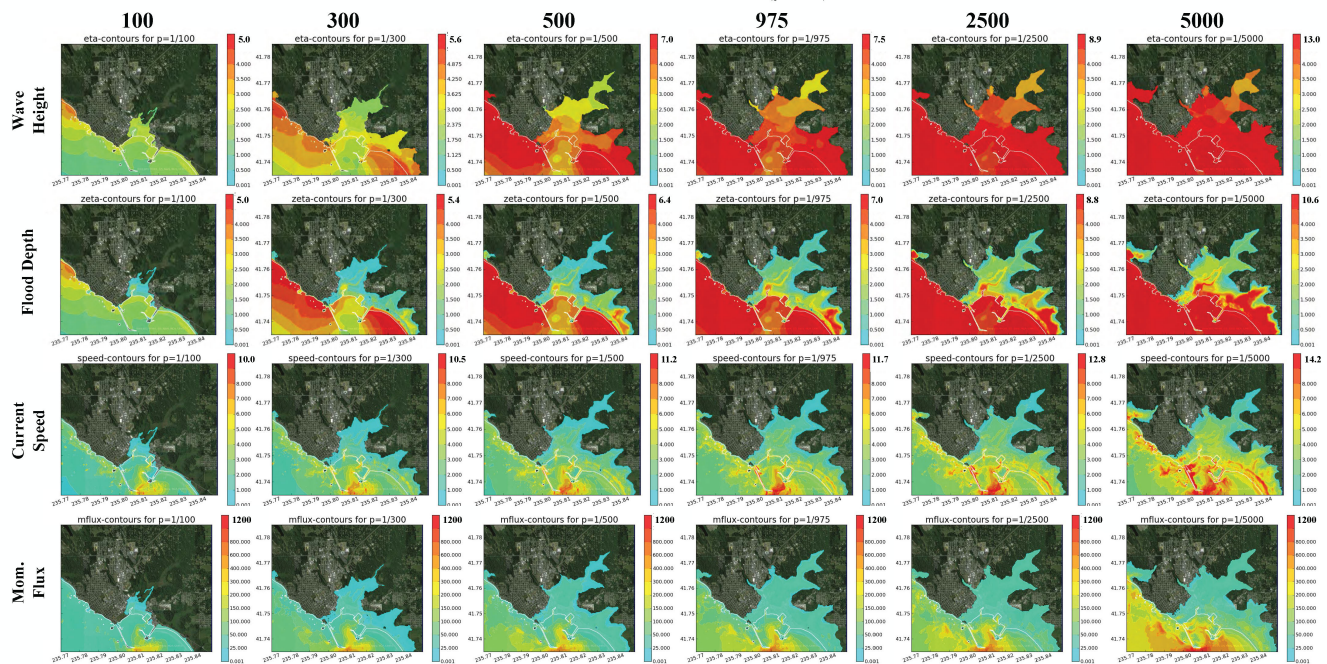
Figure 55: Wave Height, Flood Depth, Current Speed, Momentum Flux Flood Maps
