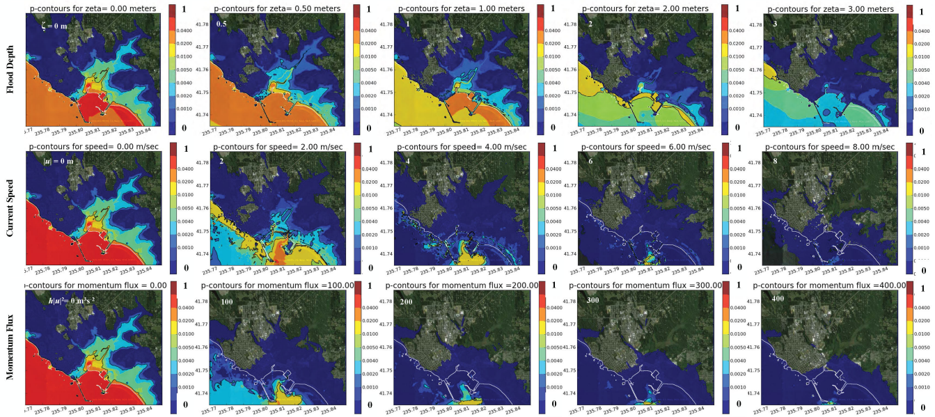
Figure 56: Flood Depth, Current Speed, Momentum Flux p-contours
