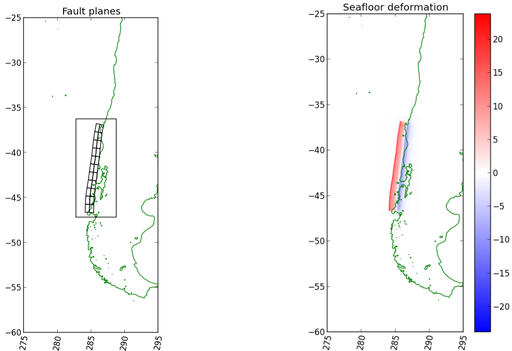
Figure 25: The sources SChSZe01. Left: Fault planes. Right: Resulting seafloor deformation.
