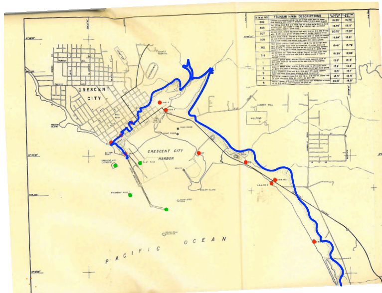
Figure 13: Inundation limits of the 1964 Alaska event tsunami, see Magoon [28].
