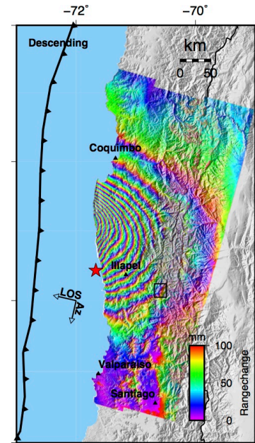
2015 Illapel earthquake
