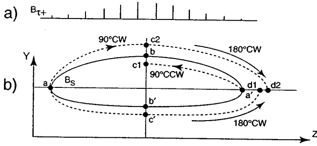
FIG. 6. (a) Axial variation of the \ell_+ = 1/2 symmetric transverse field. (b) Both 90^\circ and 180^\circ graphs of the net field (the sum of B_s , B_T , and B_\pi ) show the structure to spiral open.
