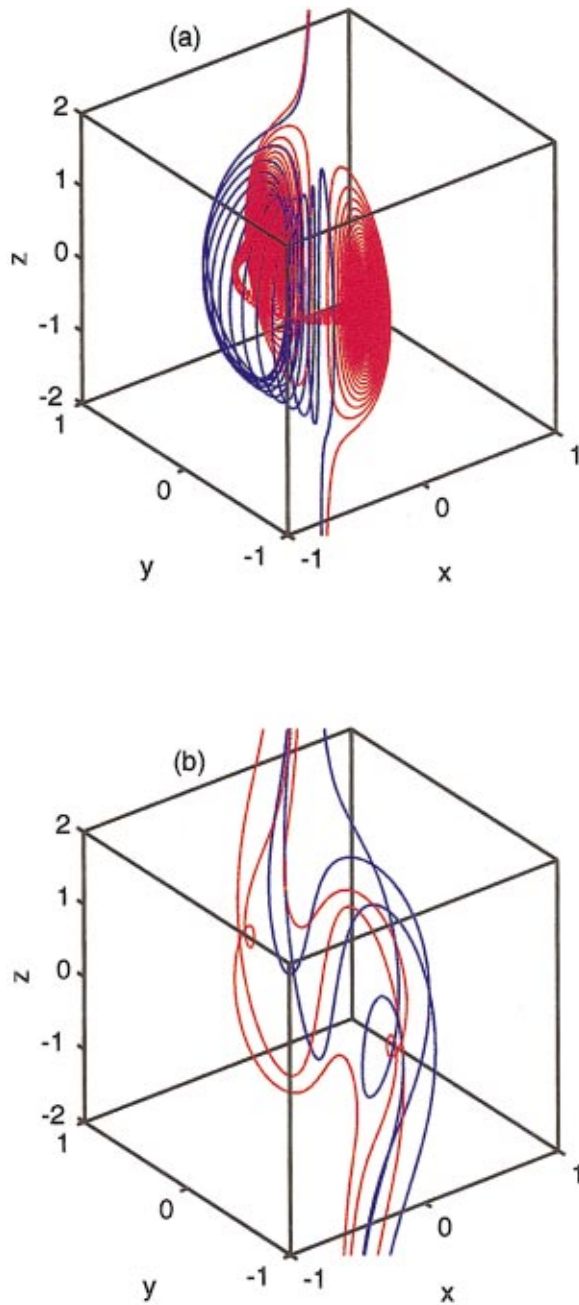
FIG. 7. (Color) (a) A small-amplitude ( B_y=0.005 ), uniform ( \ell_+=0 ), transverse magnetic field is added to a Solov'ev FRC. The red field line originates at (-0.00122, -0.7, 0) , 0.1^\circ off the y-z plane. The blue field line originates at (-0.35, -0.606, 0) , about 30^\circ from the y-z plane. Though both field lines are long, they are clearly open. (b) A larger amplitude ( B_y=0.1 ) uniform ( \ell_+=0 ) transverse magnetic field is added to a Solov'ev FRC. The red field lines originate on the x axis at x=-0.6, 0, 0.6 , and y=z=0 . The blue field lines originate on the y axis at y=-0.6, 0, 0.6 , and x=z=0 .
