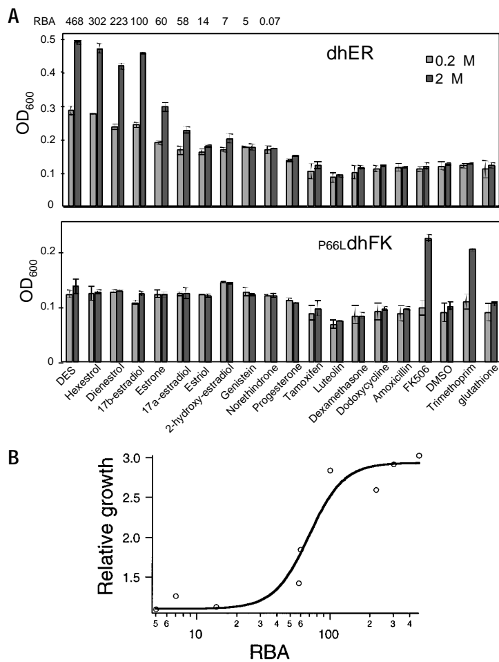
Figure 5. Chemical screen. (A) Yeast strains expressing dhER (top) or P66LdhFK (below) were screened against 20 compounds for growth at 38.5°C. Compounds were at 0.2 \mu M or 2 \mu M. OD 600 was determined after 38 h. Relative binding affinities (RBAs) for binding of estrogen analogs to ER \alpha (ref. 18) are shown at top, with estrogen (17 \beta -estradiol) at an RBA of 100. Error bars represent the deviation of two replica points of an experiment. (B) Correlation between RBA and growth of dhER (expressed as growth of yeast in 2 \mu M analog/growth with no analog), based on results shown in (A). Curve fit was generated by Igor-Pro (WaveMetrics, Lake Oswego, OR).
