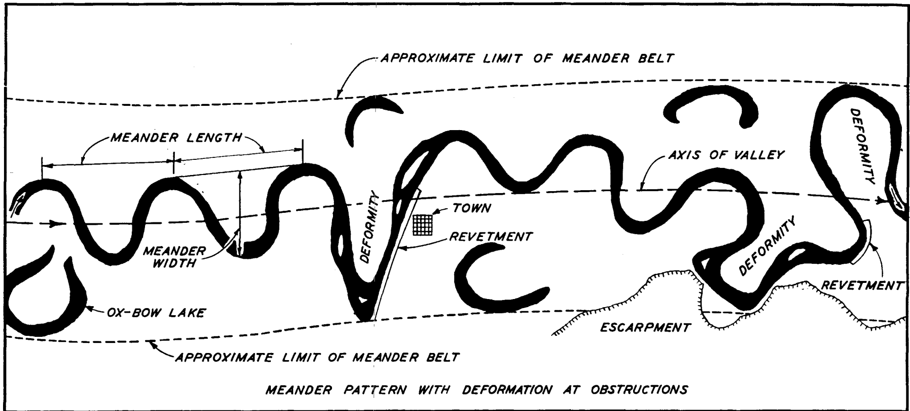
DIMENSIONS OF STREAM MEANDER RECOMMENDED BY G.H. MATTHES
