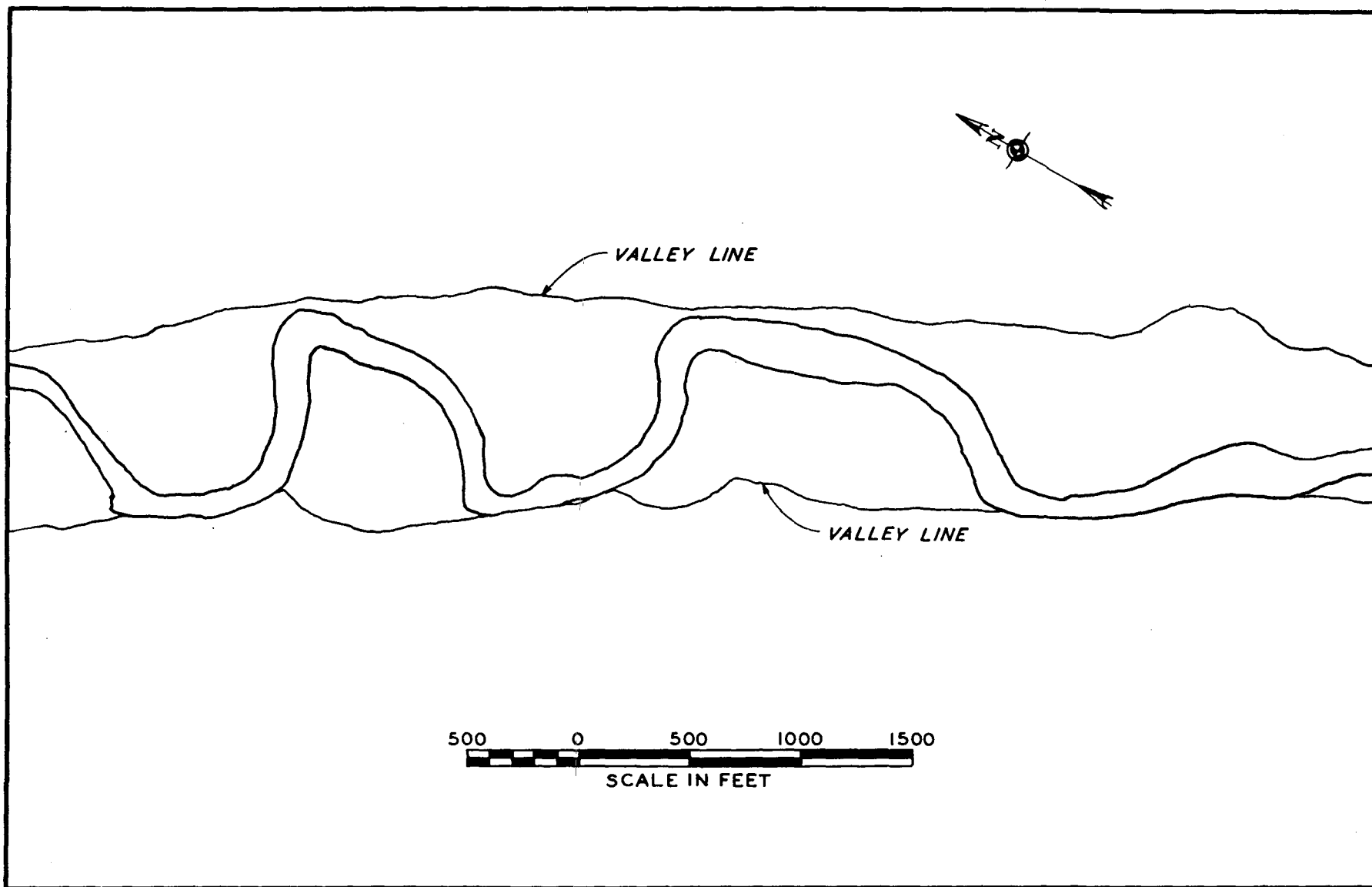
MAP OF A SECTION OF THE KLARALFVEN RIVER IN SWEDEN (A CONFINED MEANDERING STREAM)
