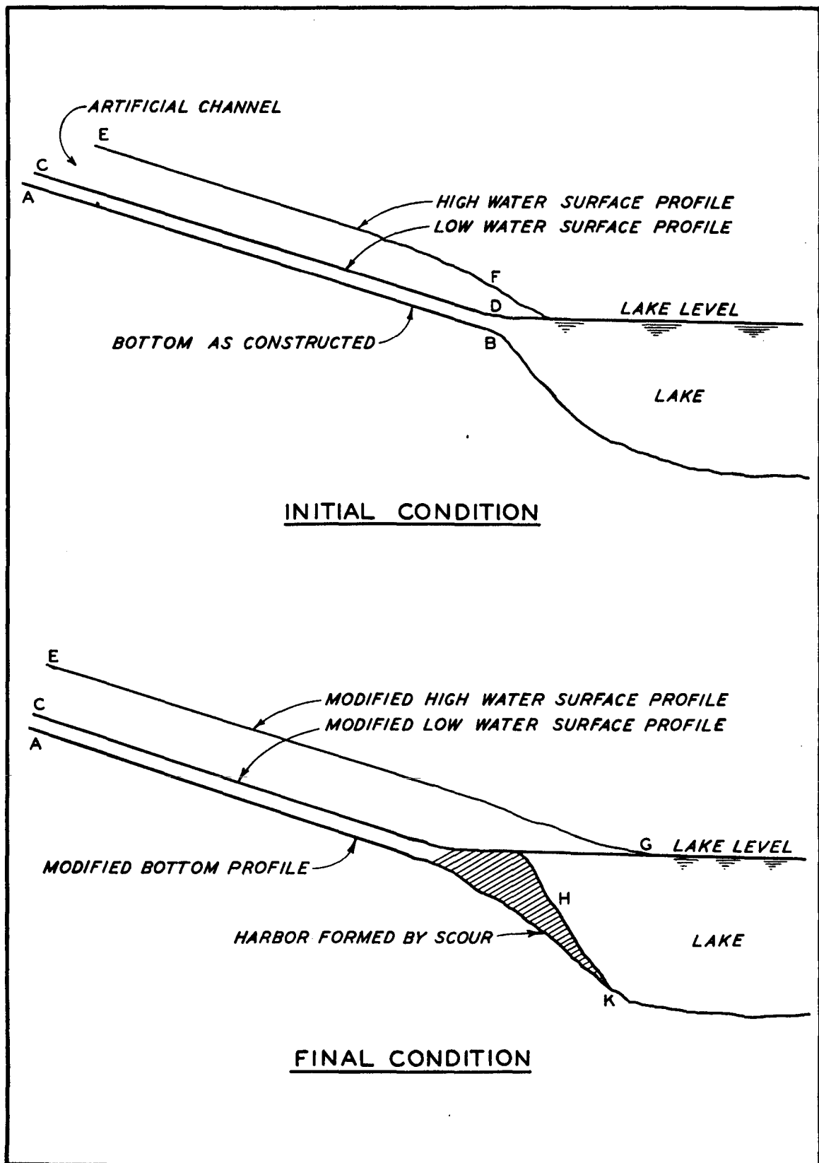
PROFILE OF ARTIFICIAL CHANNEL ENTERING A LAKE
