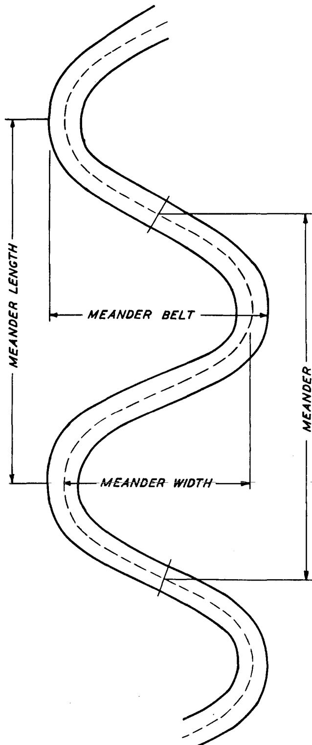
DIMENSIONS OF STREAM MEANDERS RECOMMENDED BY CENTRAL BOARD OF IRRIGATION OF INDIA
