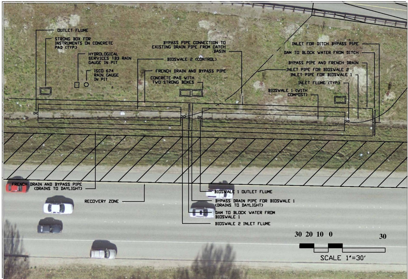
Figure 3. Site features. Photo source WSDOT Photogrammetry, date taken 3/24/2005
