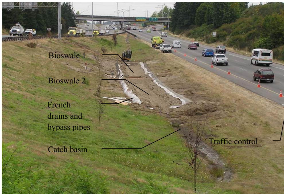
Figure 28. Bioswales ready for compost (bioswale 1) and seeding
