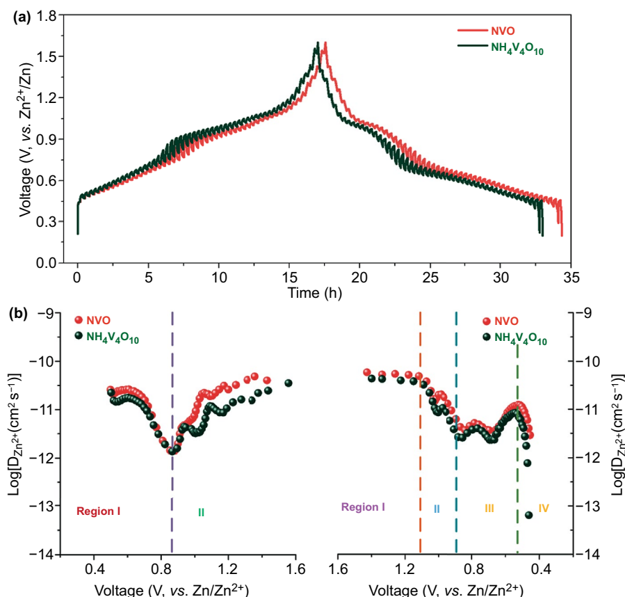
Fig. 6 Analysis of ions insertion/extraction process. a GITT tests at a current density of 50 mA h g -1 . b Corresponding ion diffusion coefficients of NVO and NH 4 V 4 O 10
