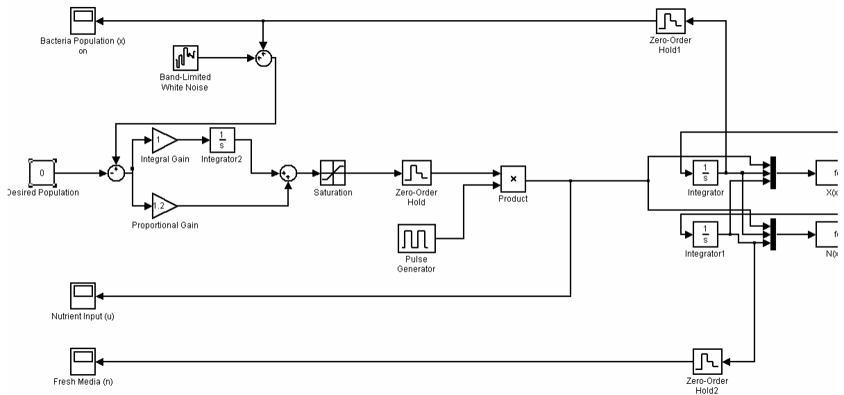
Figure 6: Simulink Model with Discrete Characteristics
