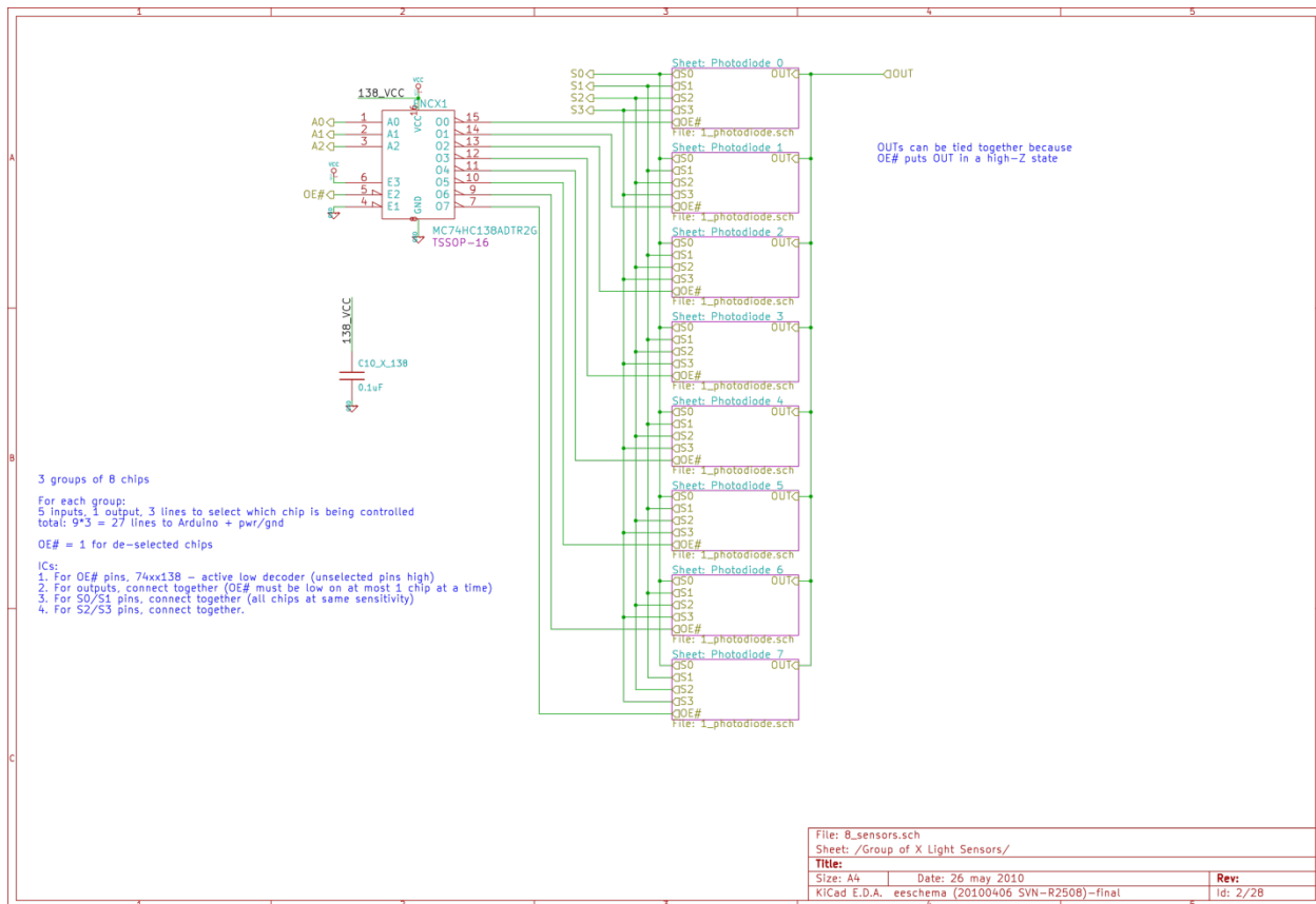
Figure 13 - The Internals of Each "Block" on Photodiode Board
