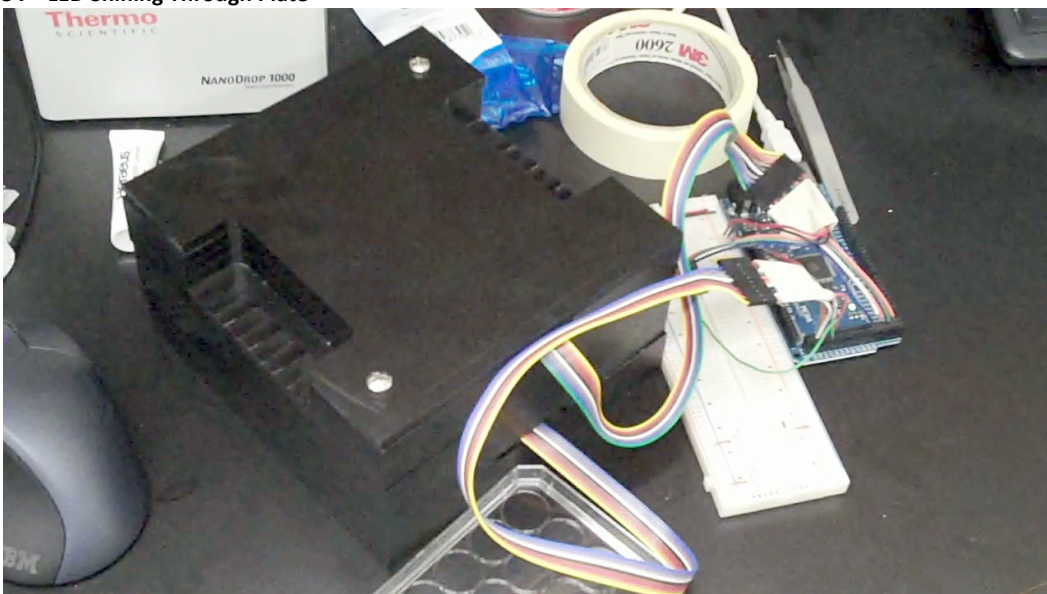
Figure 8 - View of Enclosure of Turbidostat
