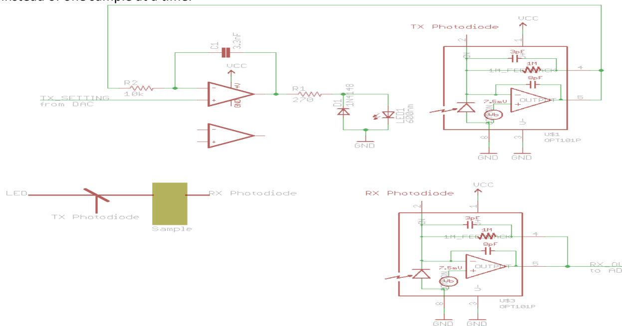
Figure 1 - Previous Turbidostat Created by Alex Leone
