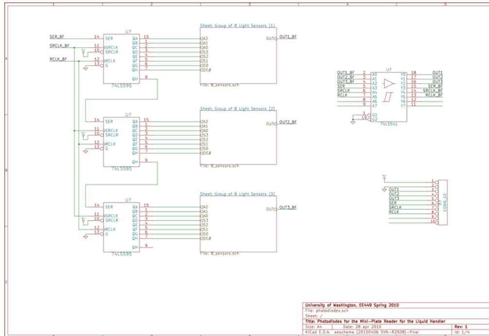
Figure 14: Photodiode circuit diagram with 8 bit shift registers
