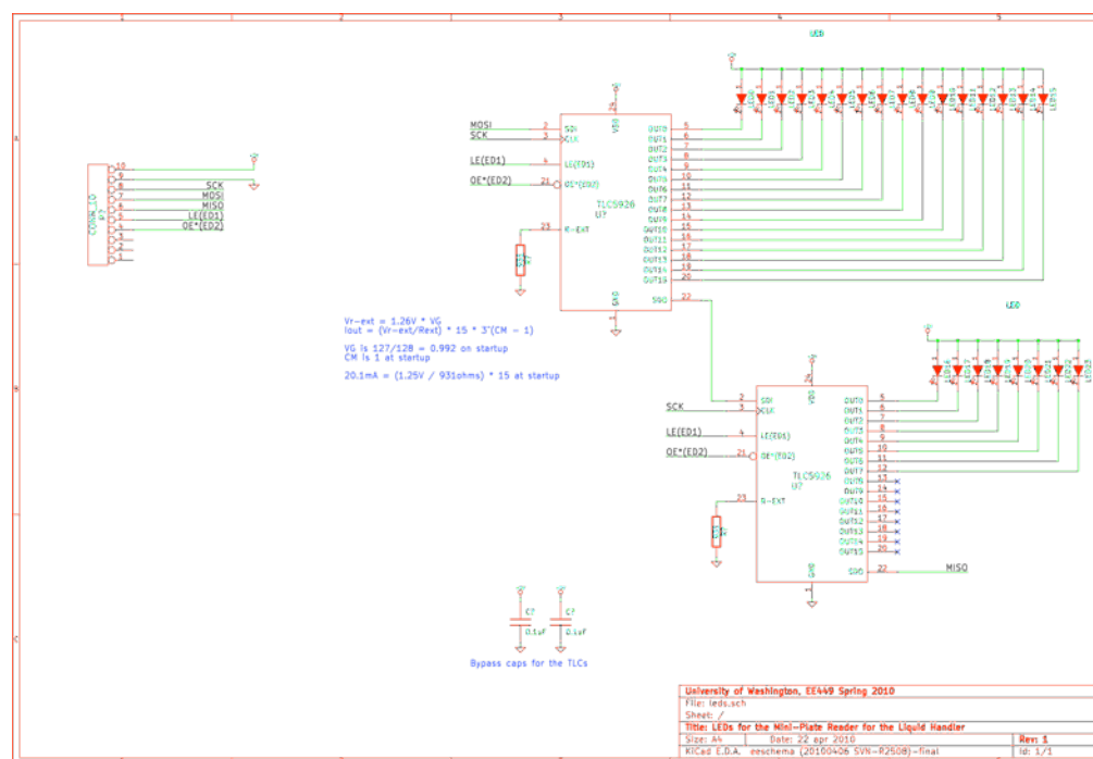
Figure 13: LED circuit diagram including current regulators
