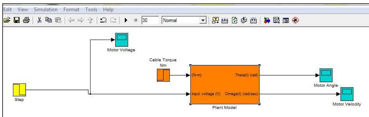
Figure 4. Simulink diagram
