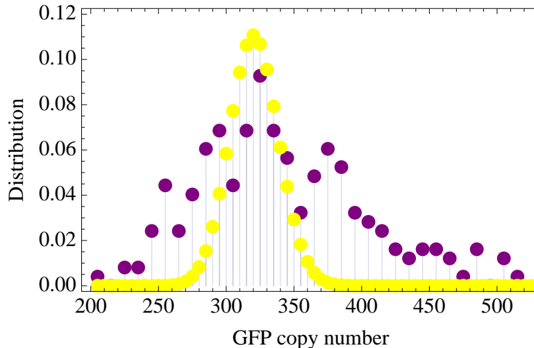
Fig. 5: GFP copy number distribution (Purple) and estimated Poisson distribution (Yellow)
