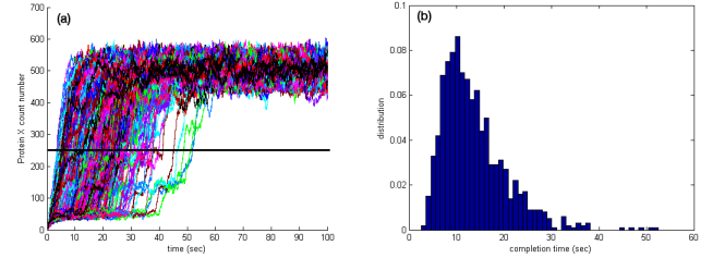
Fig. 2: (a) Thousand trajectories of the CRN obtained from the Stochastic Simulation Algorithm. (b) the approximated probability distribution of completion time (completion is when X > N , the horizontal black line in (a)). The parametric values used are [ka, \alpha, \beta_1, \beta_2, ex, dx] = [10^{-3} \log(2), 0.1, 10, 1, 10 \log(2), \log(2)] and the initial condition is [G_{unbound}, G_{bound}, X] = [5, 0, 0] .
