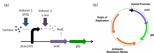
Fig. 3: A diagram of a synthetic positive feedback gene regulatory network. (a) The pLac/ara hybrid promoter is induced by IPTG and arabinose. IPTG inhibits the LacI repression of the promoter, whereas arabinose forms a complex with AraC protein and activates the promoter. (b) The network has a hybrid promoter, controlling the expression of araC and gfp downstream, an origin of replication and an antibiotic resistance marker.
