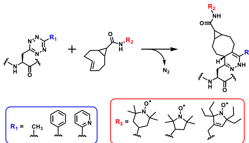
Scheme 1. Conjugation Reaction between Encoded Tet4-Amino Acids and sTCO-Spin Labels
