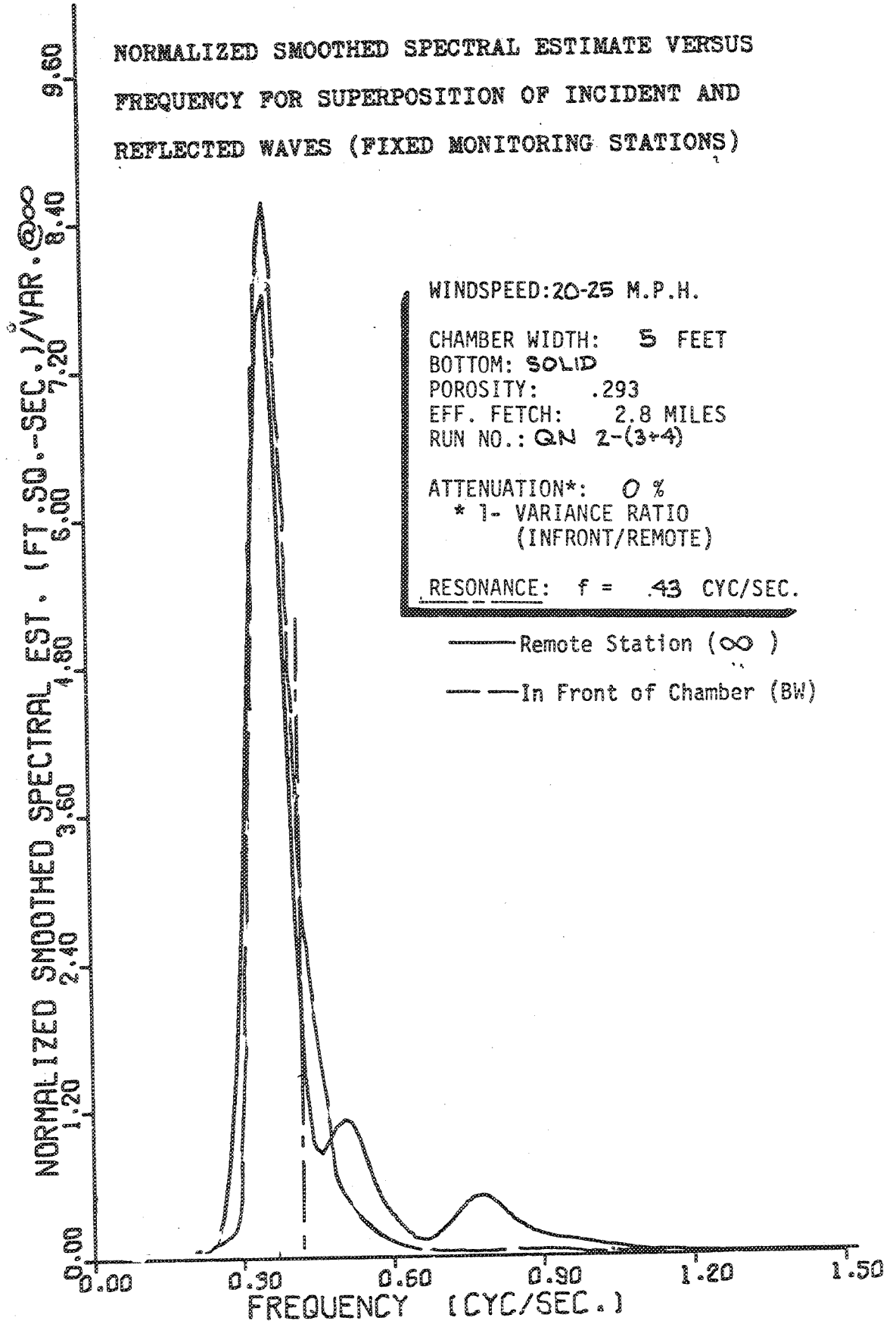
FIGURE 39. SPECTRAL PLOT FOR NYQUIST FREQUENCY EXAMPLE
