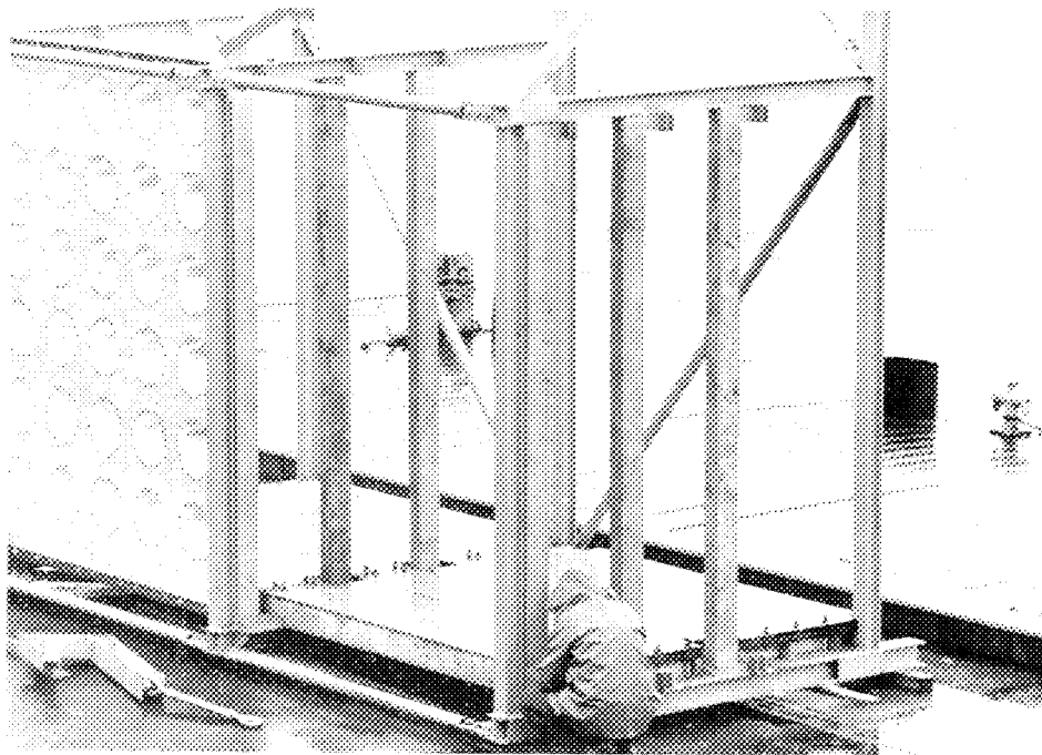
Figure 24 Removable Chamber Bottom Installed on one Module. (One porous wall panel removed; hook and turnbuckle in foreground).
