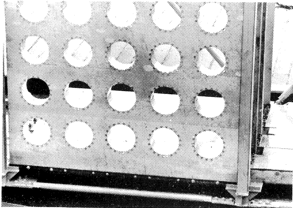
Figure 22 Porous Wall
