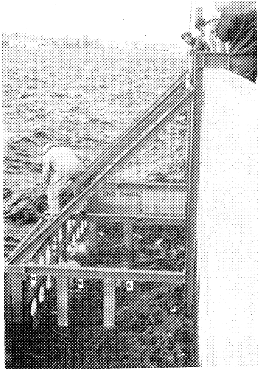
* TEST SECTION CANTILEVER BEAM ASSEMBLY RECEPTACLES
