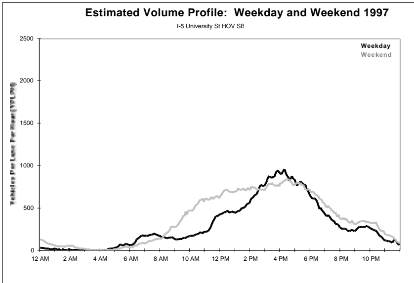
Figure 39. 1997 Weekday vs. Weekend Estimated Volume Profiles for Selected Sites
