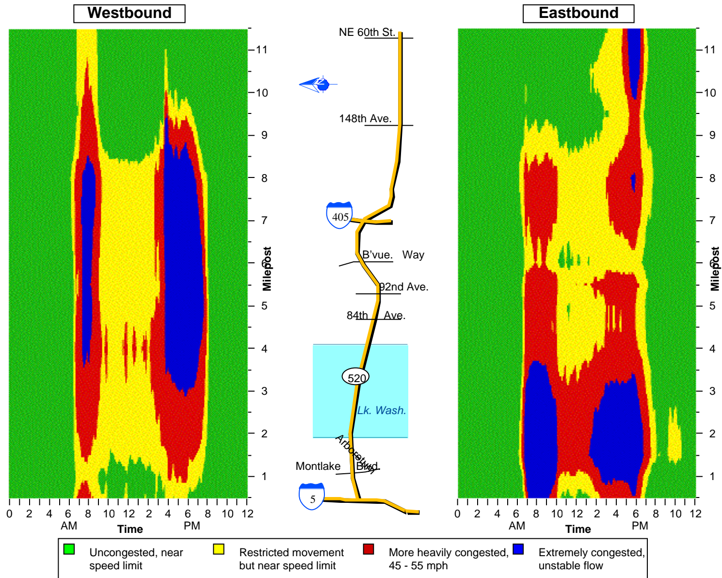
Figure 8. SR 520 Traffic Profile: General Purpose Lanes, 1997 Weekday Average
