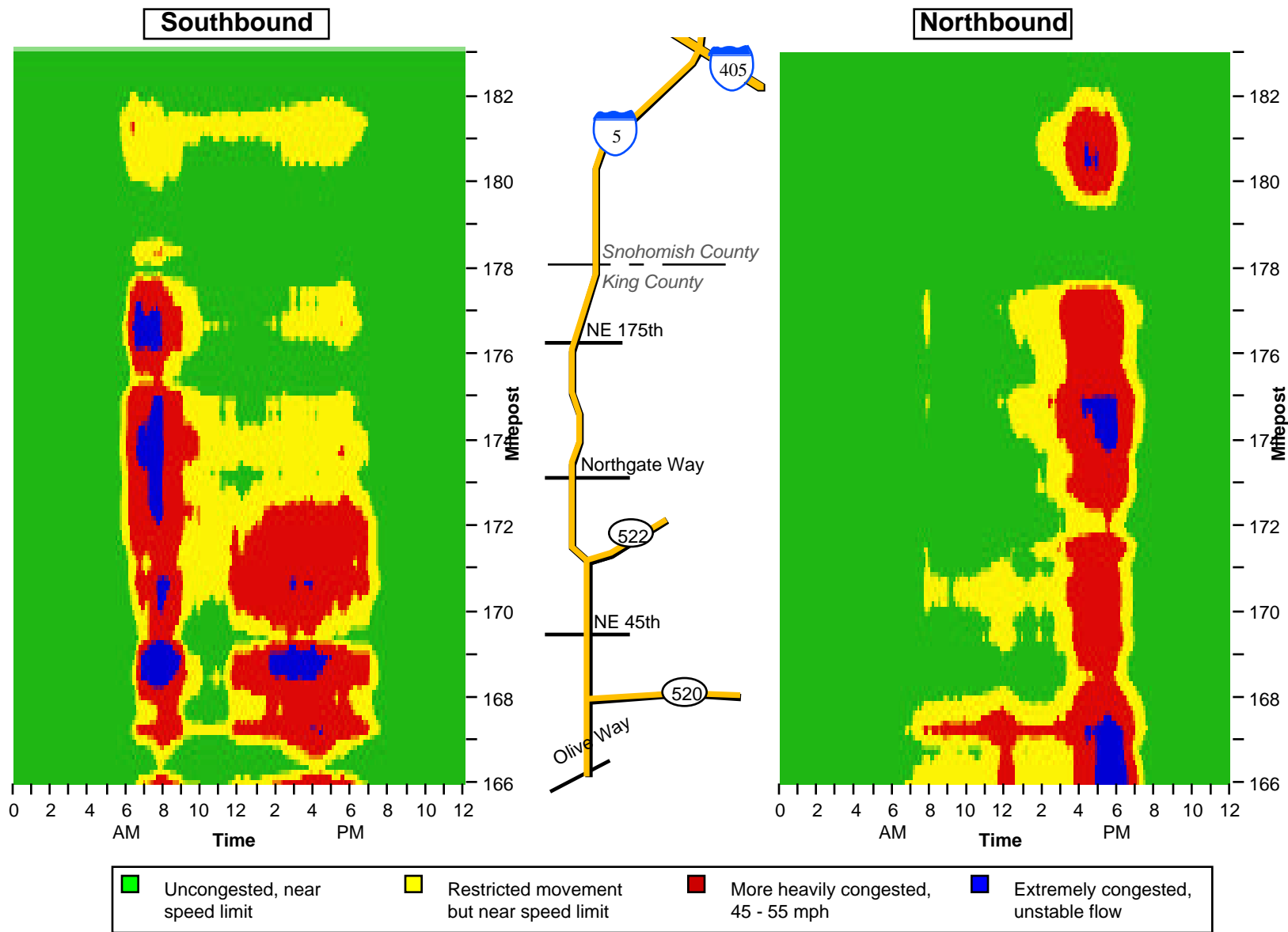
Figure 4. Interstate 5 Traffic Profile: General Purpose Lanes, 1997 Weekday Average
