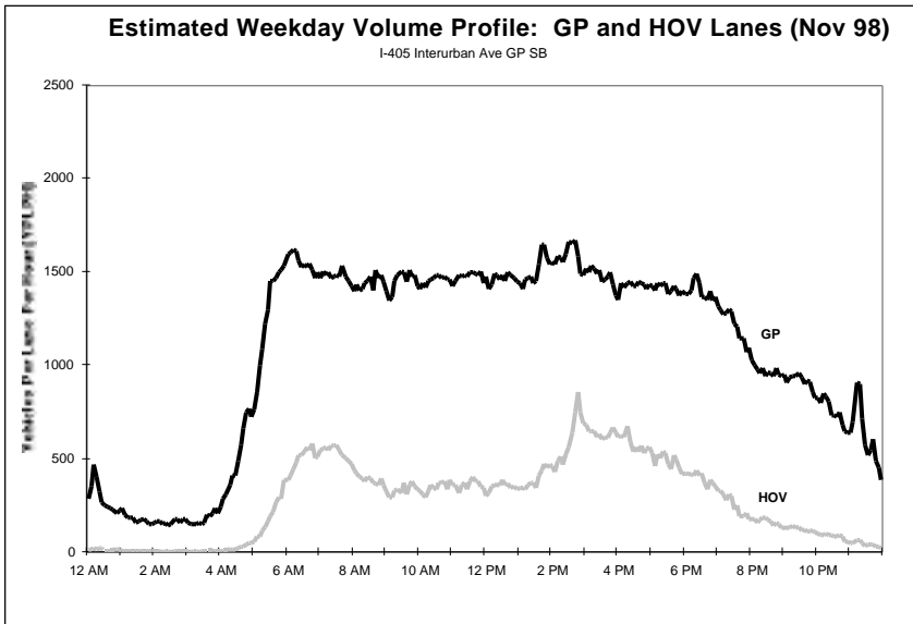
Figure 50. Estimated Weekday Volume Profiles for Selected I-405 Locations
