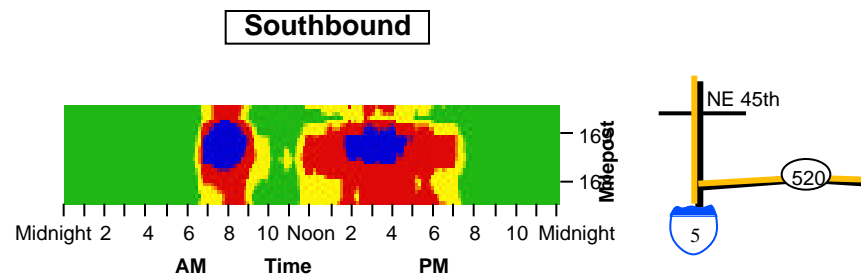
Figure 3. Traffic Profile: Southbound I-5 Ship Canal Bridge
