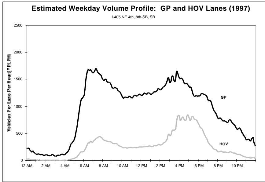
Figure 41. 1997 General Purpose vs. HOV Lane Estimated Volume Profiles for Selected Sites
