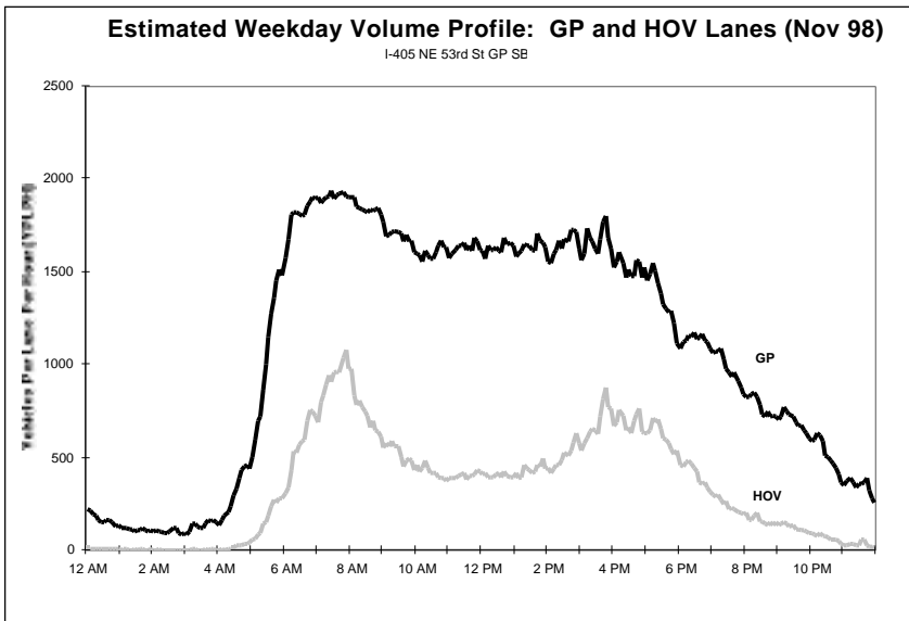
Figure 52. Estimated Weekday Volume Profiles for Selected I-405 Locations
