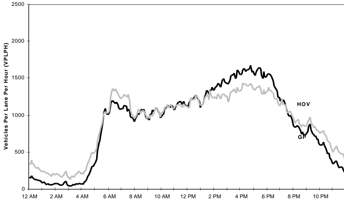
Figure 8. Estimated Weekday Volume Profile: GP and HOV Lanes
