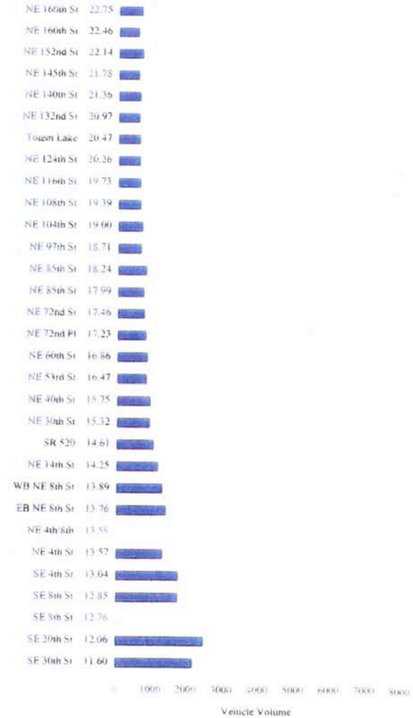
Figure 3-1. HOV Traffic Flow Profile (Nov-Dec, 1998): I-405 North of I-90 Interchange During the AM Peak Period
