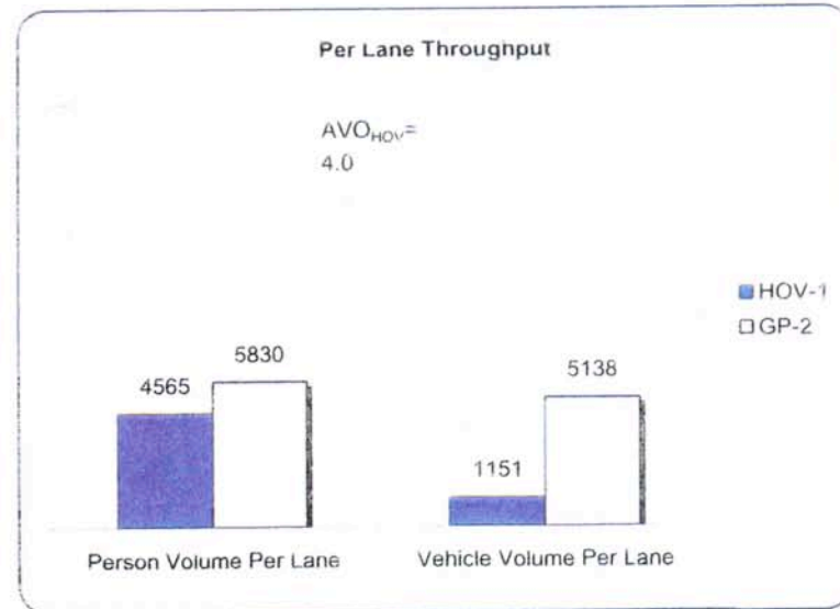
Figure 4-1. GP vs. HOV Throughput Comparison (1998): SR 520 @ 84th Ave NE
