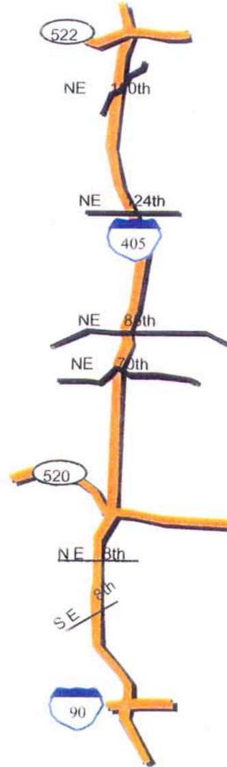
Figure 3-1. HOV Traffic Flow Profile (Nov-Dec, 1998): I-405 North of I-90 Interchange During the AM Peak Period
