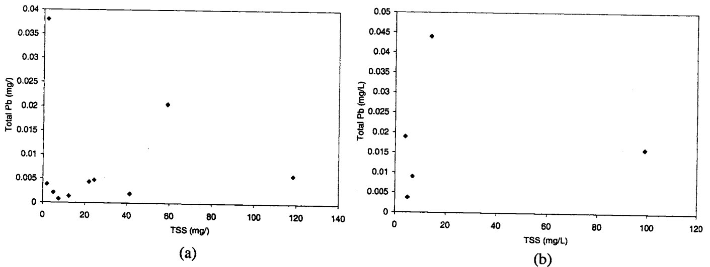
Figure 8. Total Pb concentration as a function of TSS for test plot influent (slot drain) (a) and TP1 subsurface discharge (b).
