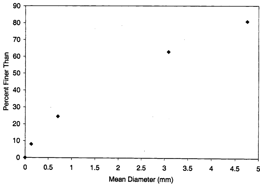
Figure 10. Particle size distribution for the sediment retained in the slot drain collection system.
