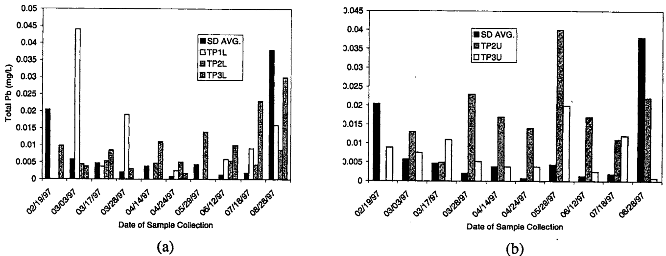
Figure 7. Total Pb concentration in the test plot influent (slot drain) and test plot subsurface (lower) collection points (a) and surface (upper) collection points (b).
