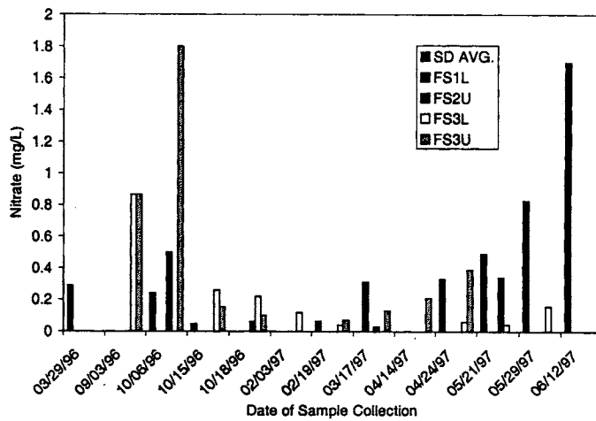
Figure 14. Nitrate concentration data for the slot drain average and test plots.
