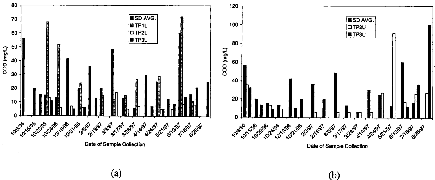
Figure 6. COD concentration in the test plot influent, surface and subsurface collection points: (a) subsurface COD concentrations, (b) surface COD concentrations.
