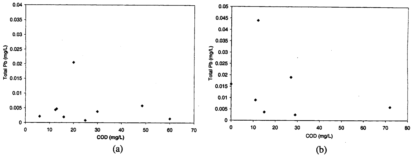
Figure 9. Total Pb concentration as a function of COD for test plot influent (slot drain) (a) and TP1 subsurface discharge (b).
