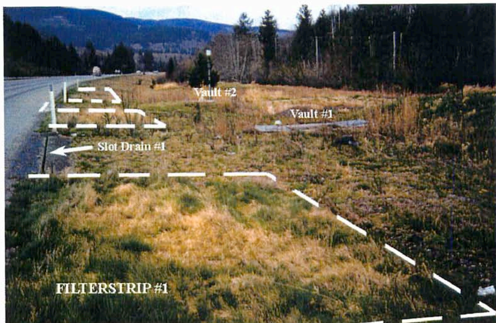
Figure 3. Photograph of the test site along SR 8 showing the sample vaults, test plots, and slot drain #1.
