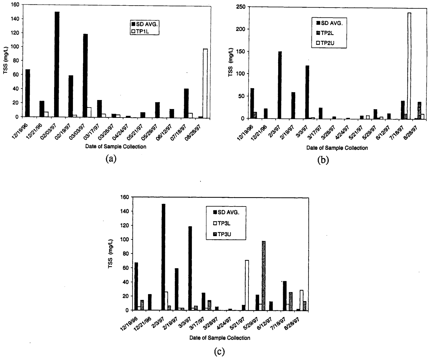
Figure 5. TSS values for test plot 1, 2, and 3 compared to the slot drain (test plot influent) averages. TP2L and TP2U refers to test plot 2 lower (subsurface) collection and upper (surface) collection points, respectively.
