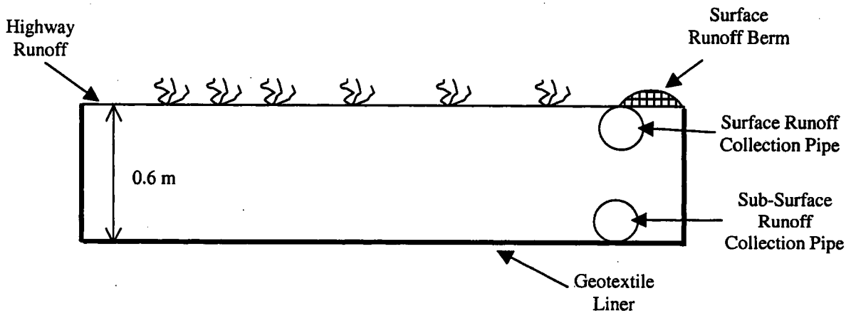
Figure 2. Cross sectional view of a test plot showing the surface runoff diversion berm and collection pipes (not to scale).
