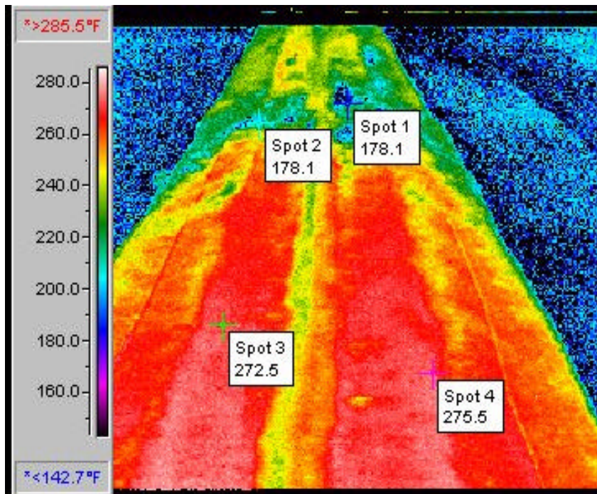
Figure A3. Infrared Image of I-5 (Blaine) 1998 Paving Project with Truck End Dumping (Note: Temperatures are in °F)
