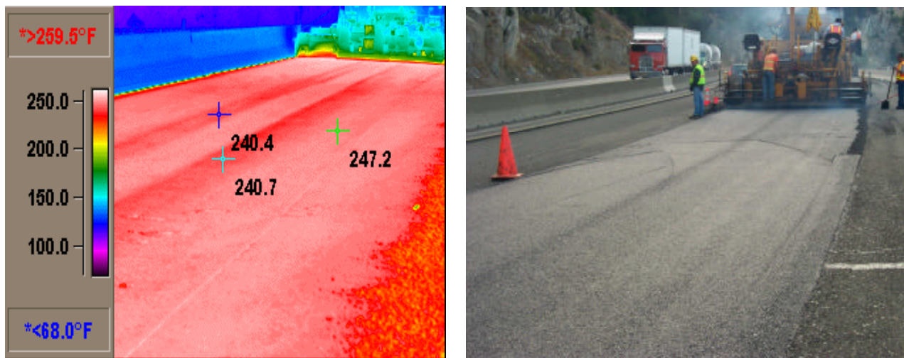
Figure 11. Infrared Image of Longitudinal Streak. Figure 12. Photo of Longitudinal Streak.
