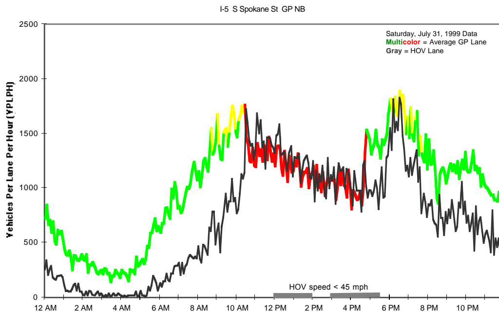
Figure 7: Estimated GP and HOV volume and speed, I-5 S. Spokane St., general purpose lanes northbound
