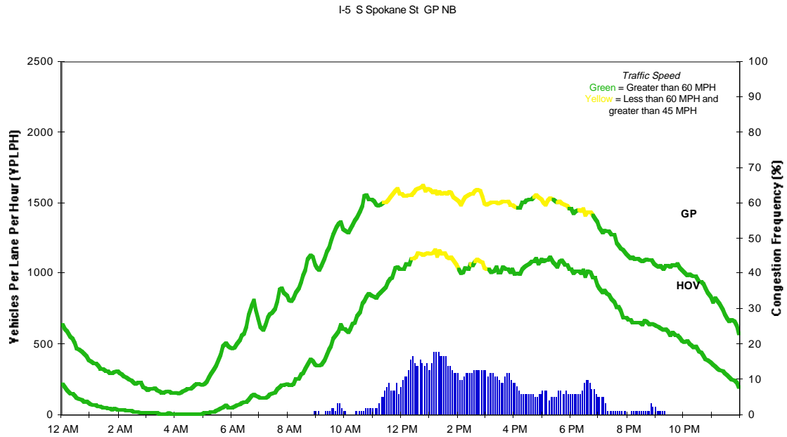
Figure 6: Estimated weekend volume, speed, and reliability conditions (1999), I-5 S. Spokane St., general purpose lanes northbound
