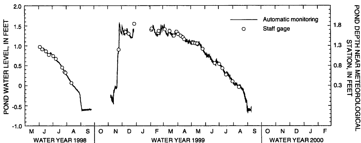
Figure 4. Water level of pond in the gypsum-treated retention basin, and depth of the pond near the site of the meteorological station near DuPont, Washington, June 1998 to September 1999.
