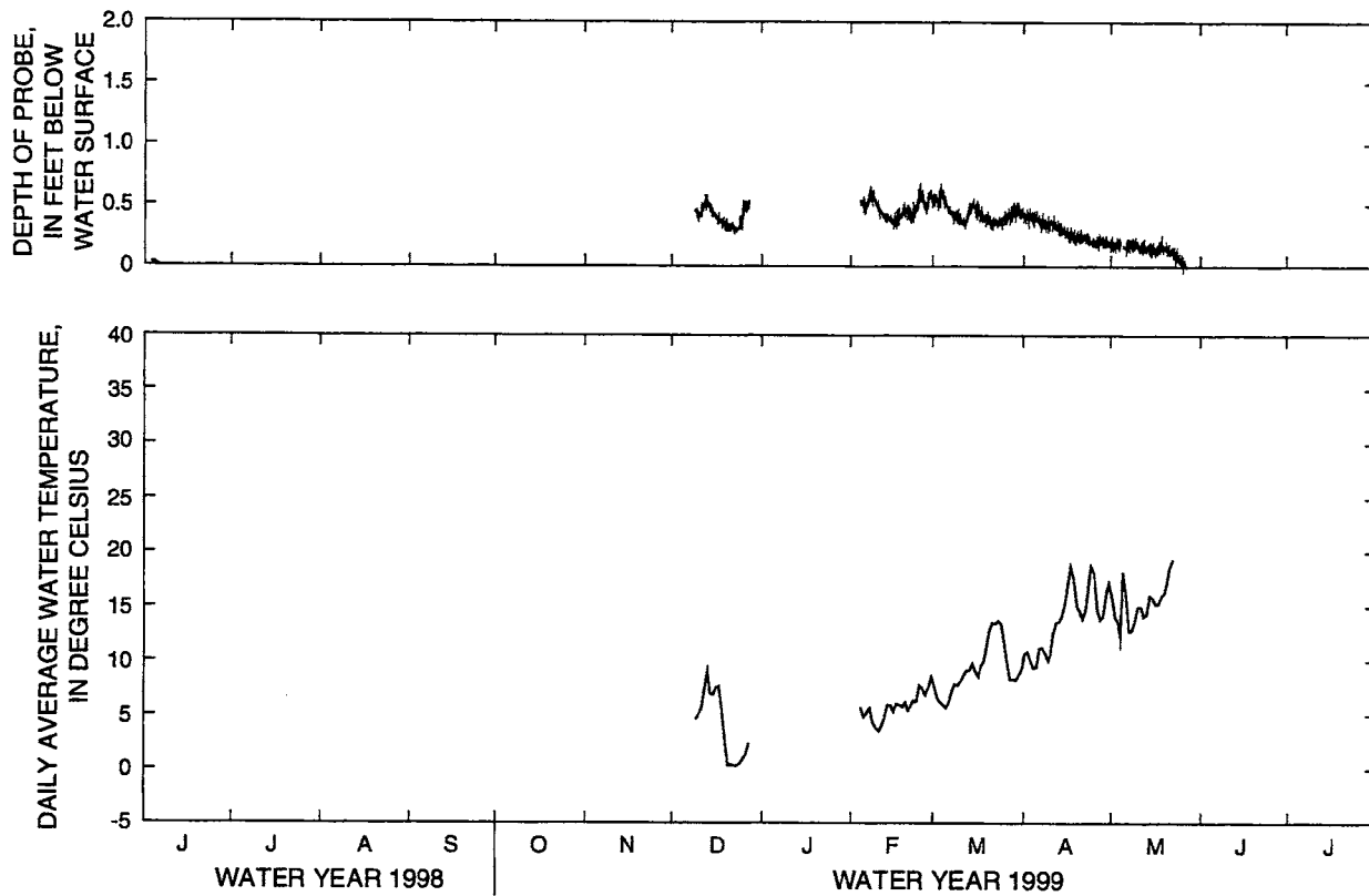
B. Depth of the highest post-mounted soil/water temperature probe (#2) and daily average water temperature
