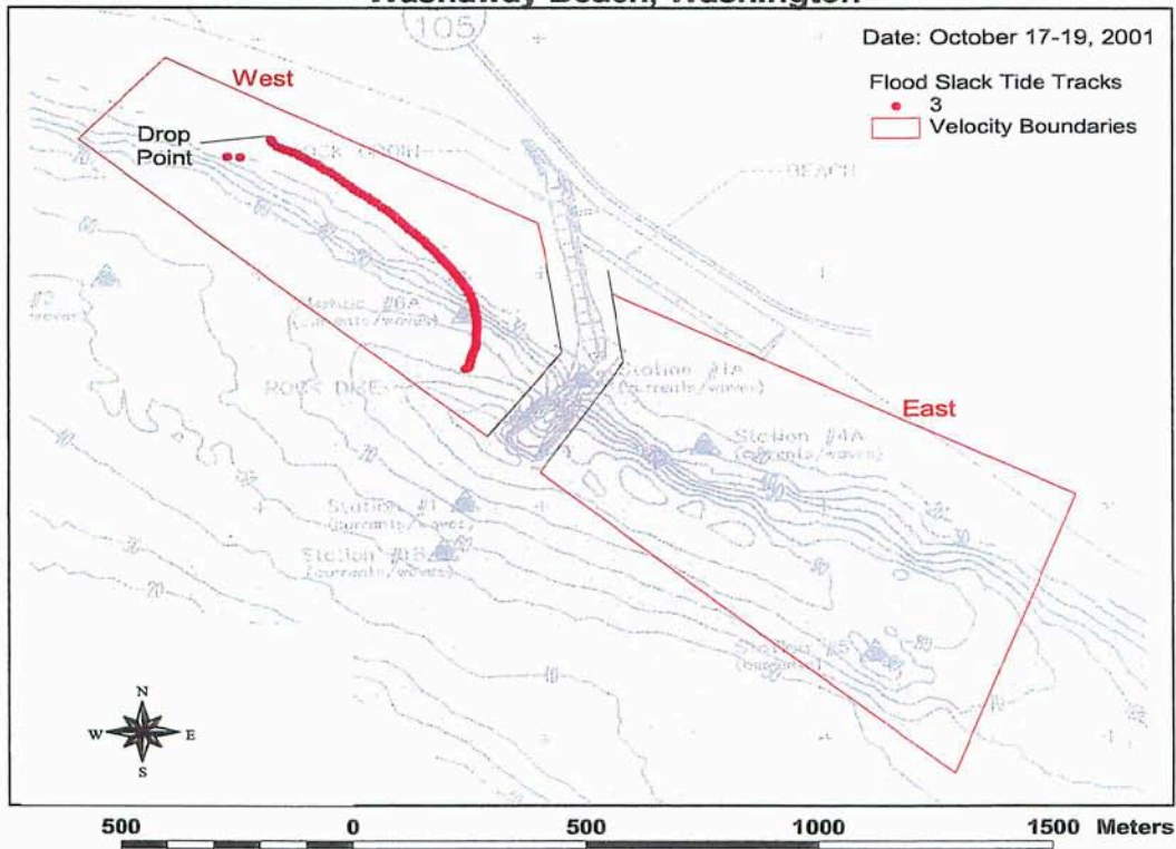
Figure 6. Drift buoy track recorded as a flood tide turned slack tide at Washaway Beach, Washington.
