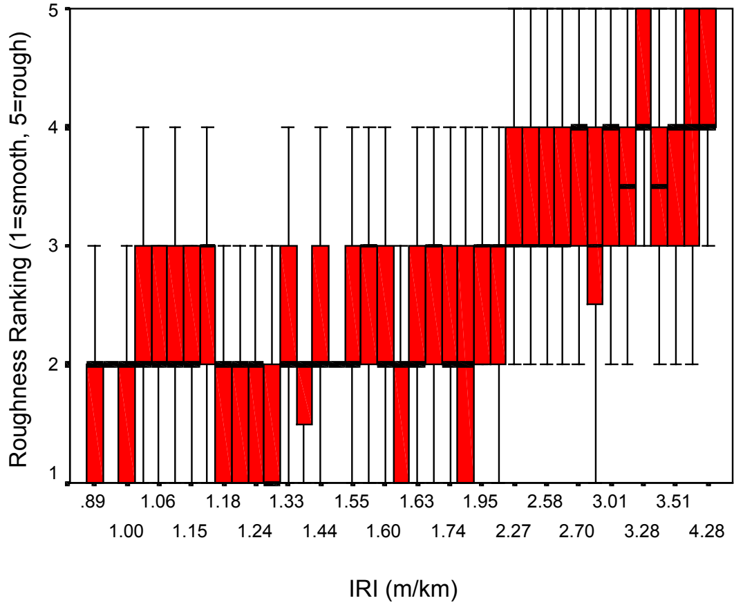
Figure F-1. Boxplot of Roughness Ranking vs. Measured IRI (m/km)
