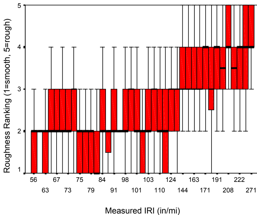
Figure 12. Boxplot of Roughness Ranking vs. Measured IRI
