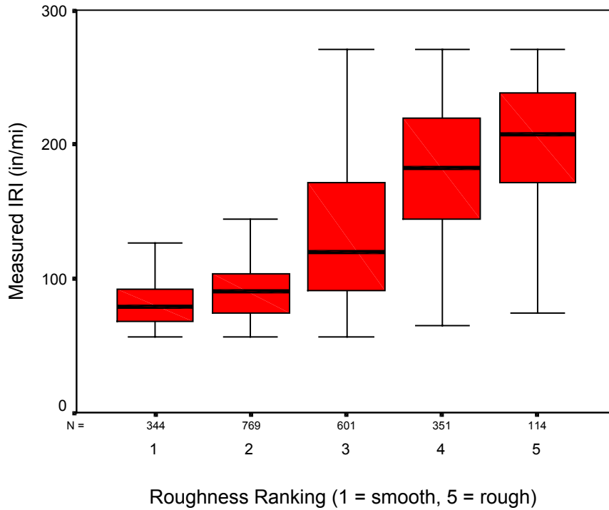
Figure 14. Boxplot of IRI vs. Roughness Ranking
