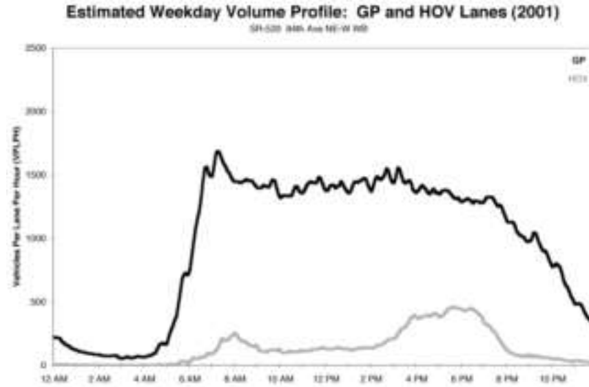
Figure 5.7. Estimated Weekday Volume Profile: GP and HOV Lanes (2001), SR 520 at 84th Ave NE, Westbound
