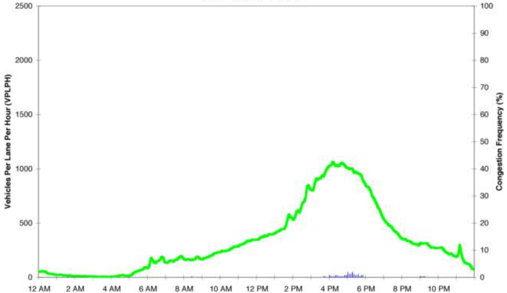
Figure 4.20. Estimated Weekday Volume, Speed, and Reliability Conditions (2001): Southbound SR 167, South 34th St, HOV Lane
