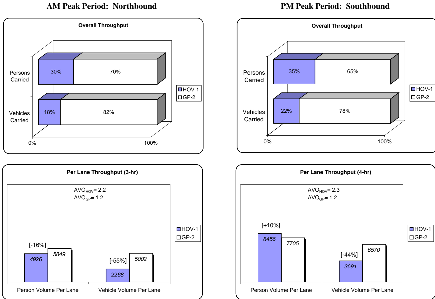
Figure 2-40. GP vs. HOV Throughput Comparison (2002): SR 167 near Kent
