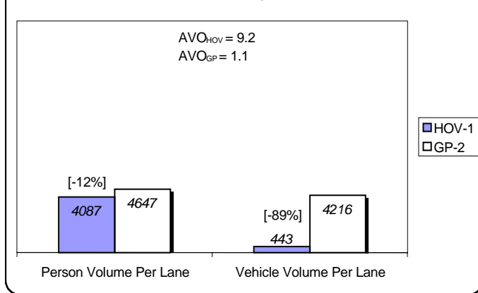
Figure 2-39. GP vs. HOV Throughput Comparison (2002): SR 520 near Median
