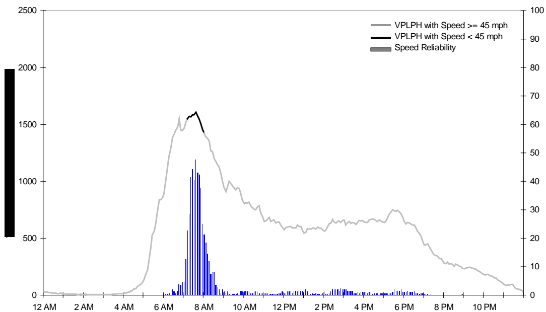
Figure 3-20. Average Weekday Volume, Speed, and Reliability Condition: I-5 @ NE 145 th St
