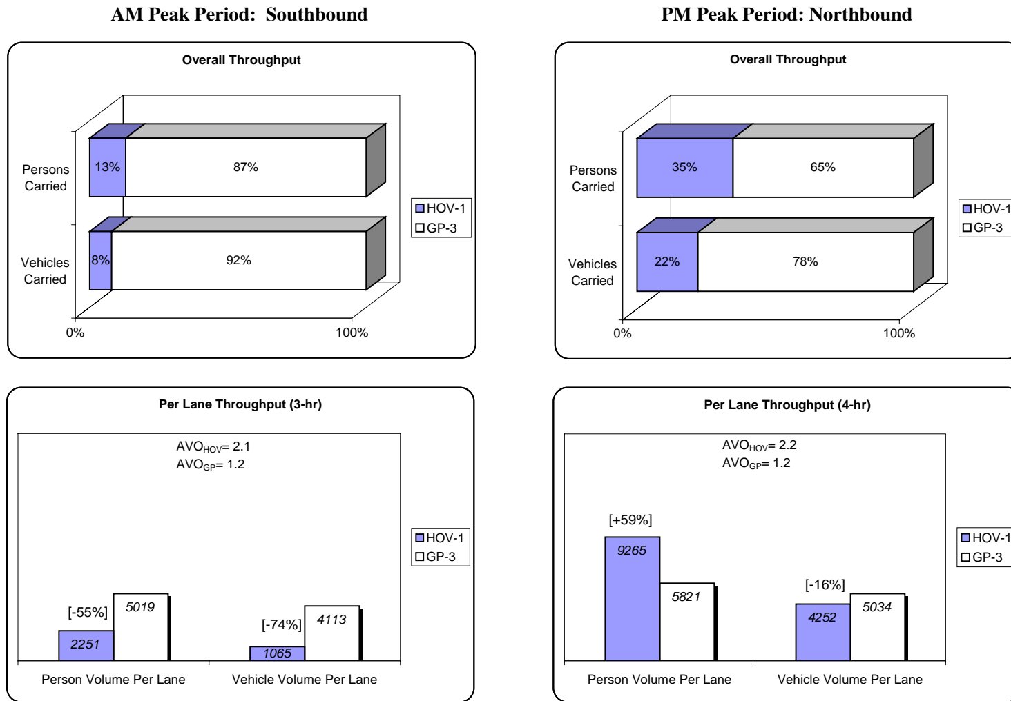
Figure 2-36. GP vs. HOV Throughput Comparison (2002): 1-405 near Southcenter
