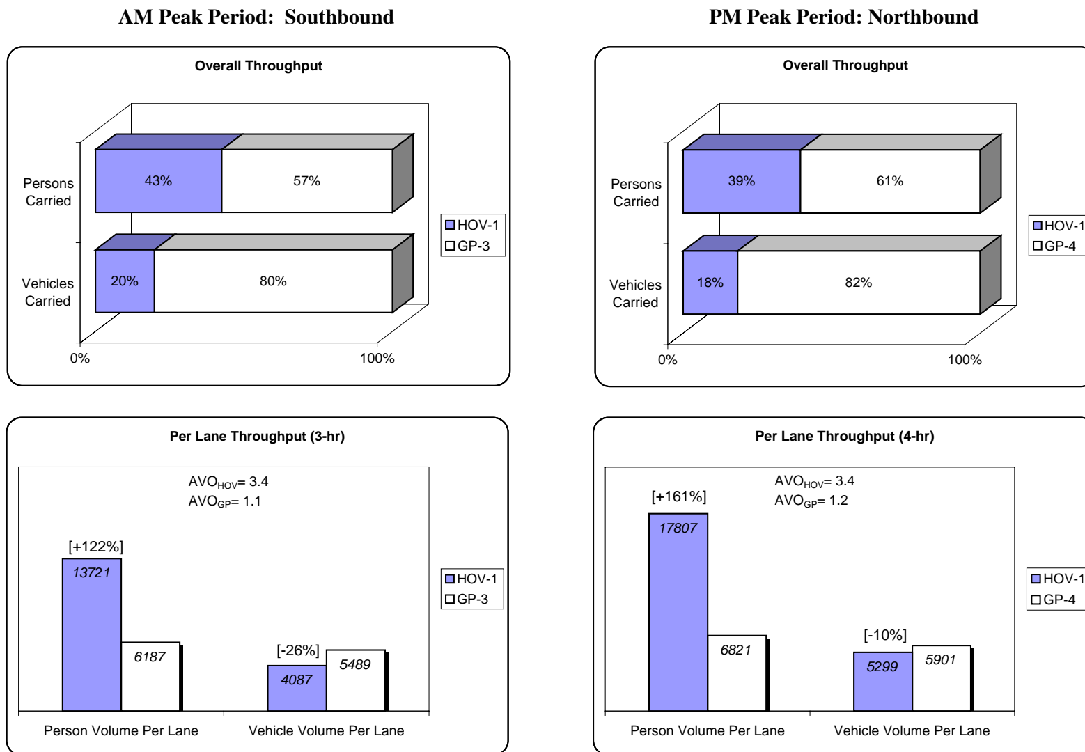
Figure 2-31. GP vs. HOV Throughput Comparison (2002): 1-5 near Northgate
