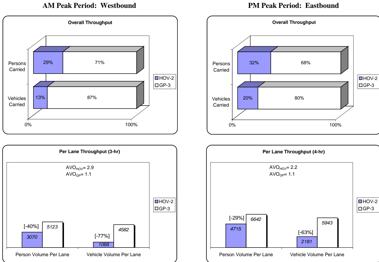
Figure 2-37. GP vs. HOV Throughput Comparison (2002): I-90 Floating Bridge
