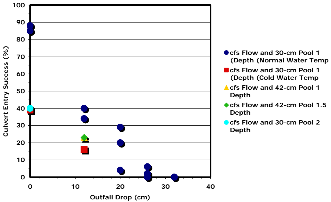
Figure 6. Culvert entry success for all tests including 42-cm pool depth, cold temperature, and higher flow tests.
