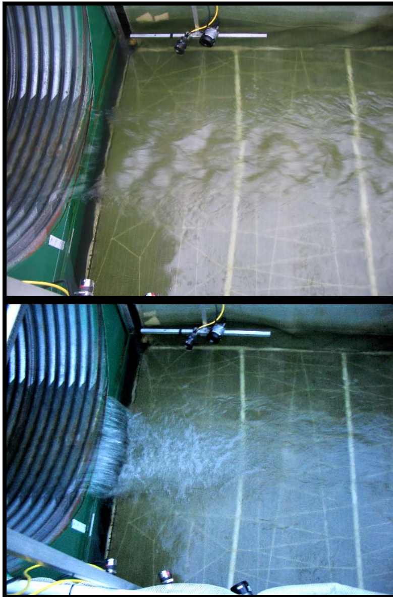
Figure 3. Culvert entrance with 0-cm outfall drop (streaming flow, top) and 12-cm outfall drop (bottom)
