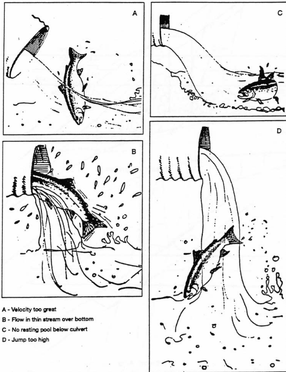
Figure 1. Examples of culvert fish-passage barrier conditions (Powers and Orsborn 1985).
