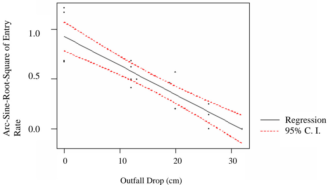
Figure 7. Regression of arc-sine-square-root transformation of the proportion of fish entering the culvert in relation to outfall drop. Dashed lines represent the 95% confidence interval for the fitted line.
