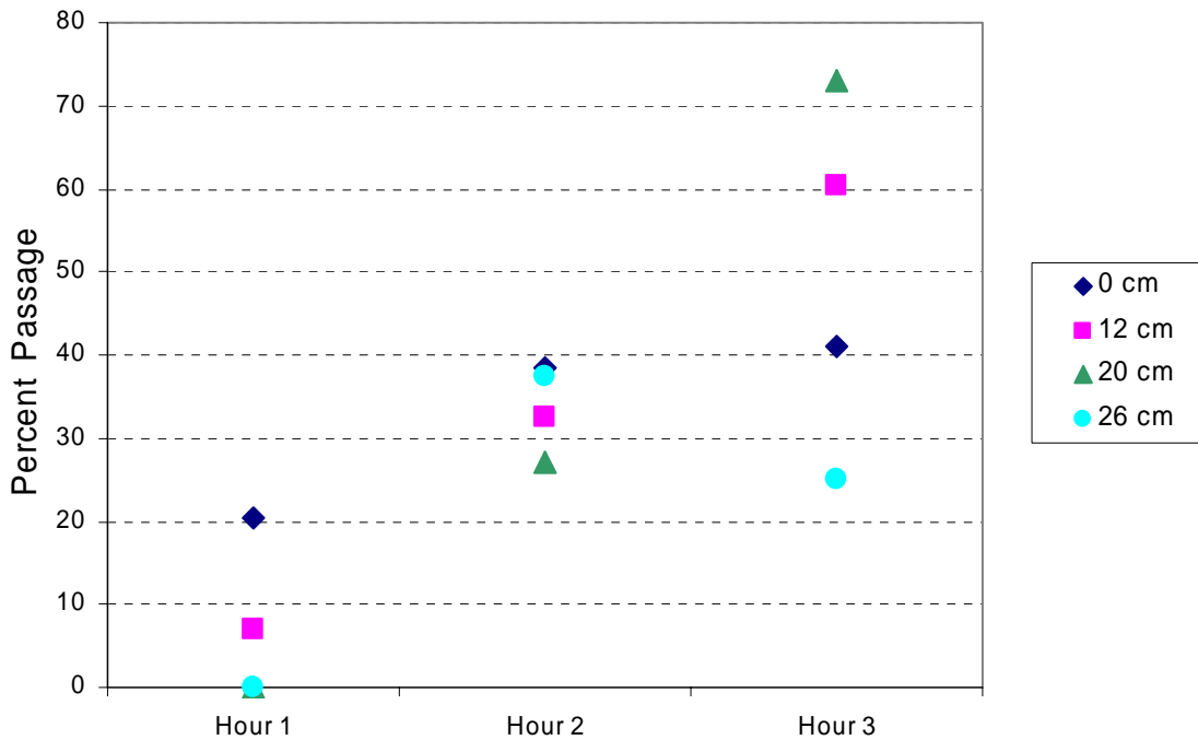
Figure 14. A qualitative estimate of hourly culvert entry rates for fish successfully entering perched culvert (n=3 for all outfall-drop conditions). Data are based on real-time observations recorded during each test.
