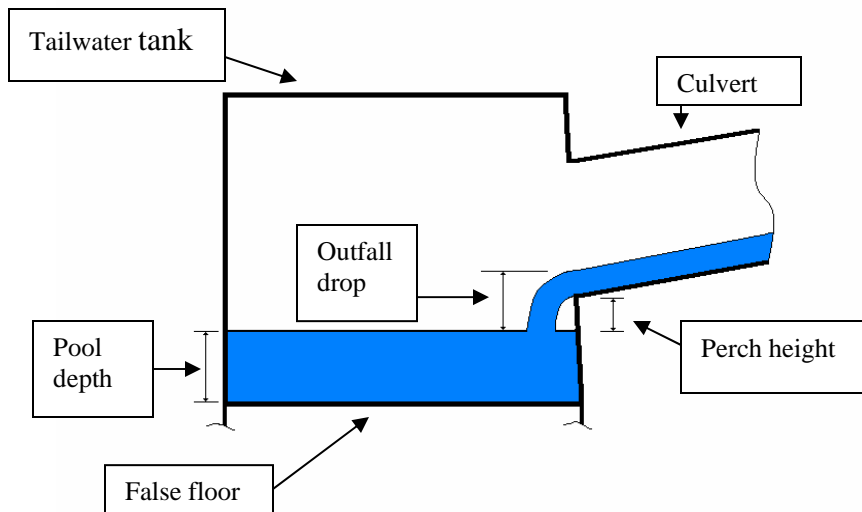
Figure 2. Diagram of culvert entrance showing outfall drop, perch height, and tailwater pool depth (net pen excluded from drawing for clarity).
