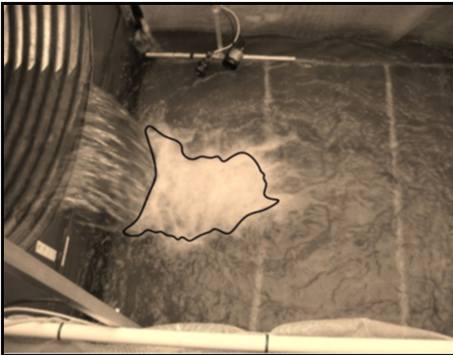
Figure 15. Photo showing extent of the turbulence zone at the 32-cm outfall drop.
