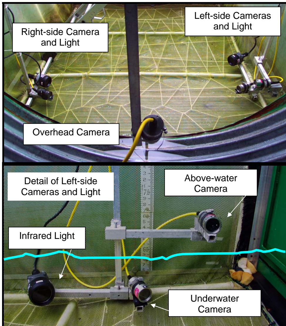
Figure 5. Cameras and infrared lighting used to observe fish behavior (blue line indicates waterline).
