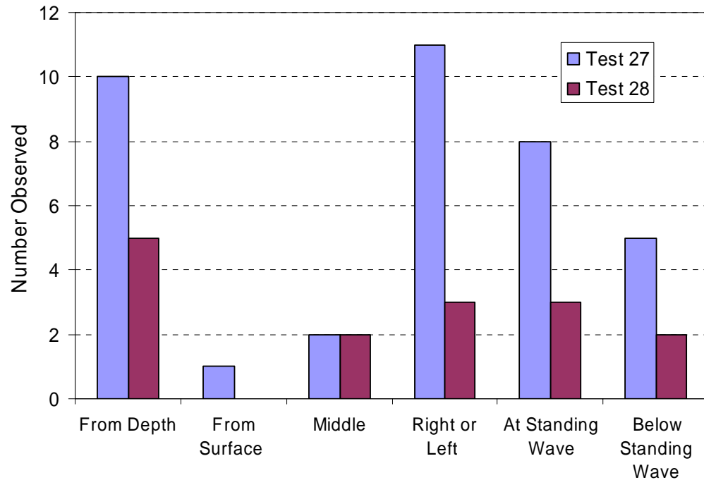
Figure 8. Summary of leaping fish for tests 27 and 28 (12 cm outfall drop) with depth of fish just prior to successful leap, and their position relative to the culvert entrance when leaping from the tailwater pool.
