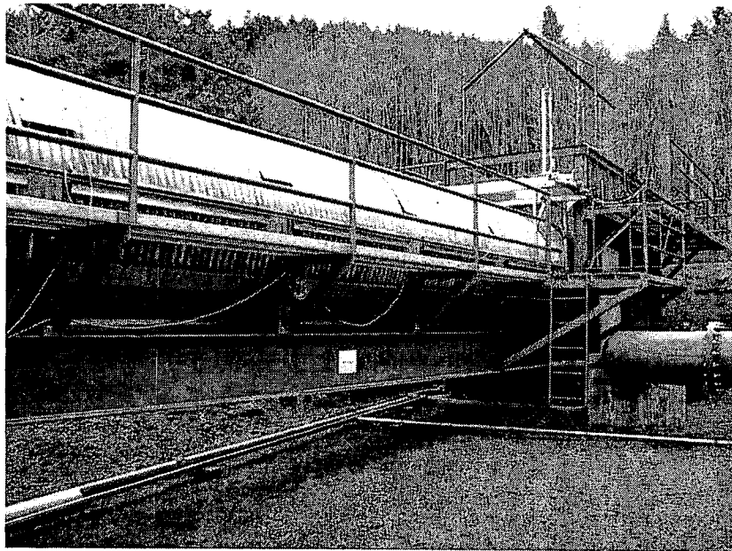
Figure 1. Culvert Test Bed. This photograph shows the culvert (foreground) and headwater tank (right side).
