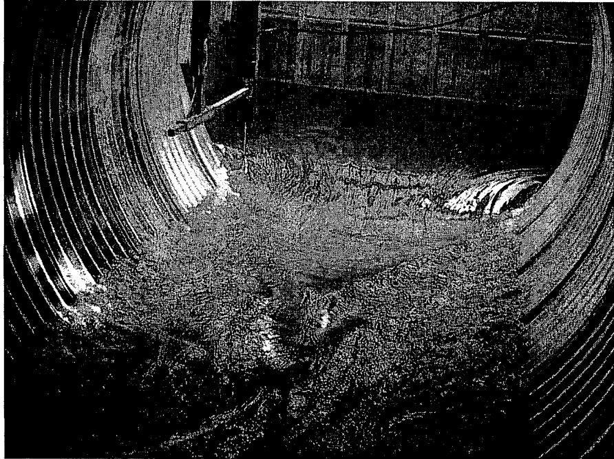
Figure 27. Picture of the Flow Conditions at the Culvert Inlet. Note that the reduced velocity zones at the culvert edges disappear near the culvert inlet at the HW tank.
