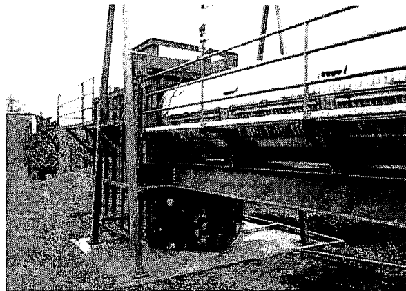
Figure 4. Culvert Test Bed Showing Tailwater Tank, A-frame, and Culvert Barrel.
