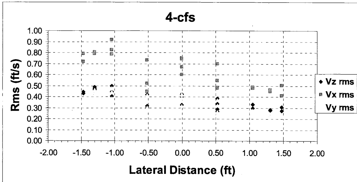
Figure 23 (cont'). Turbulence Intensities (RMS) at 3.5 and 4 cfs (station 4).
