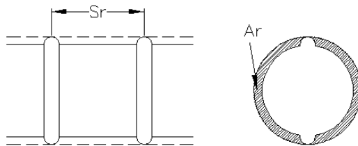
Figure 3.2: Bar dimensions for relative rib area
