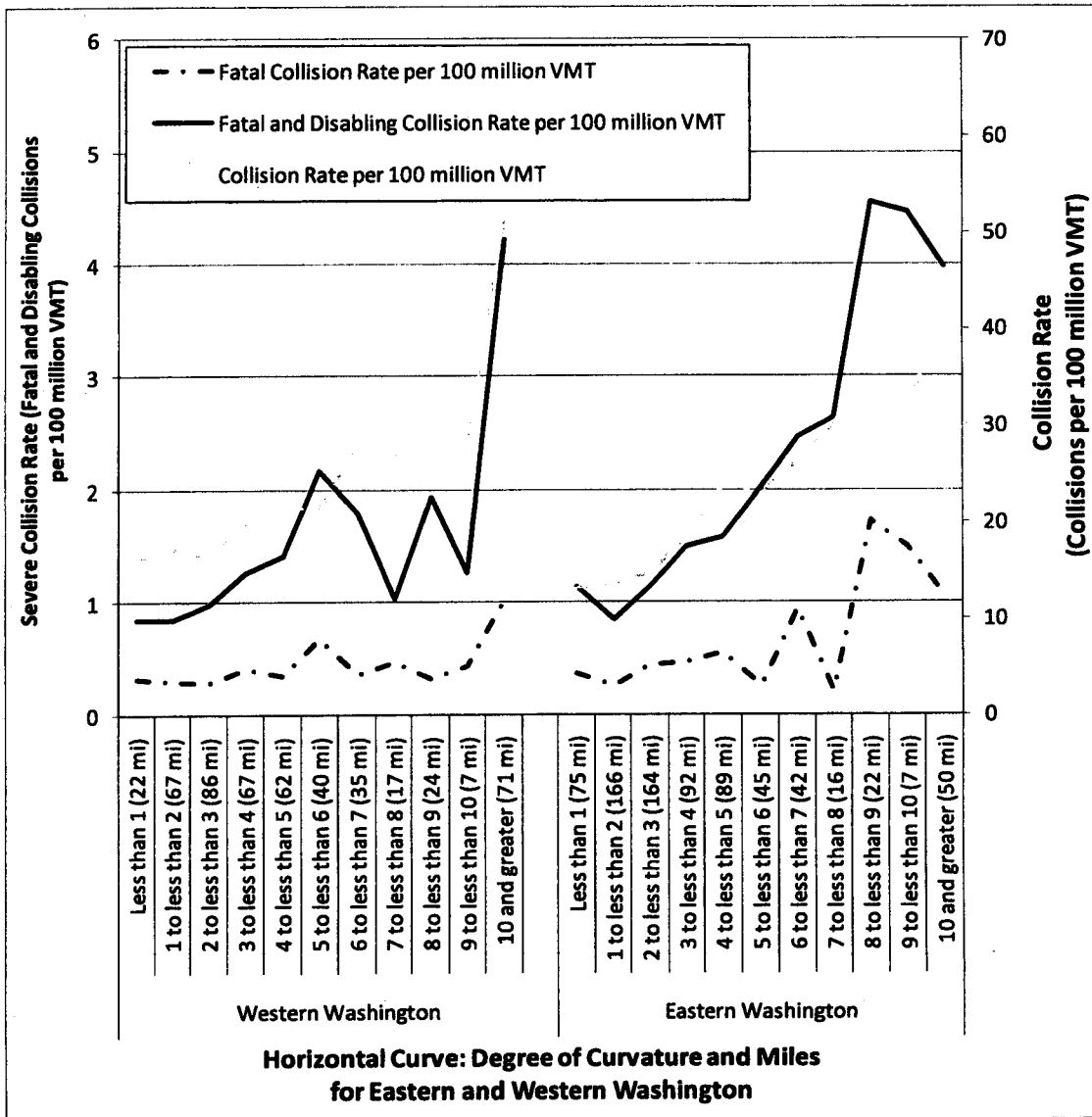
Figure 15: Evaluation of collision; fatal injury; and fatal and disabling injury collision rates for the seven-year period 1999 – 2005 for varying categories of horizontal degree of curvature and comparing eastern and western Washington
