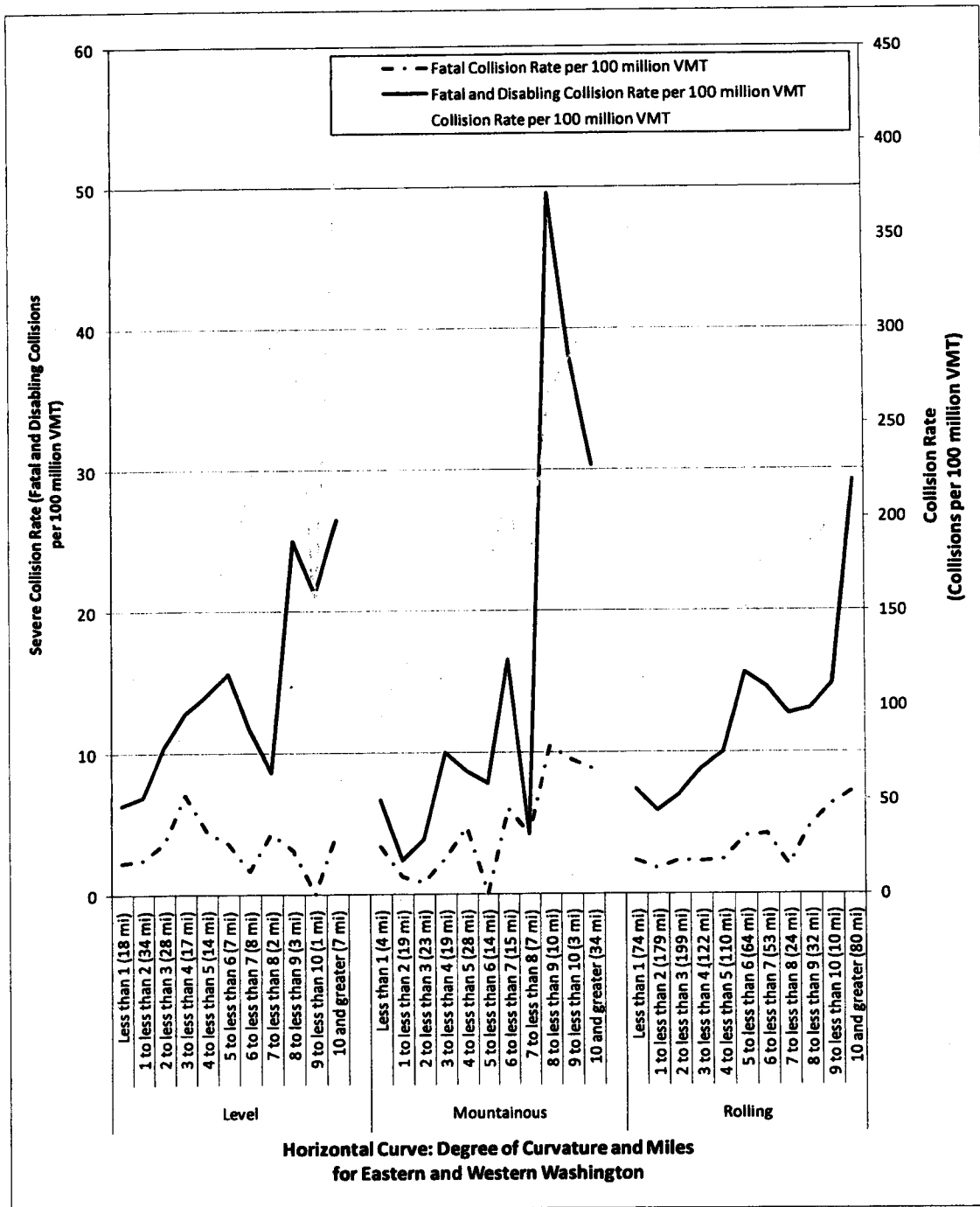
Figure 16: Evaluation of collision; fatal injury; and fatal and disabling injury collision rates on horizontal curves for the seven-year period 1999 – 2005 for different terrain types
